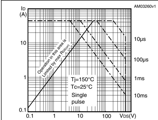
Figure 8. Safe operating area for DPAK
