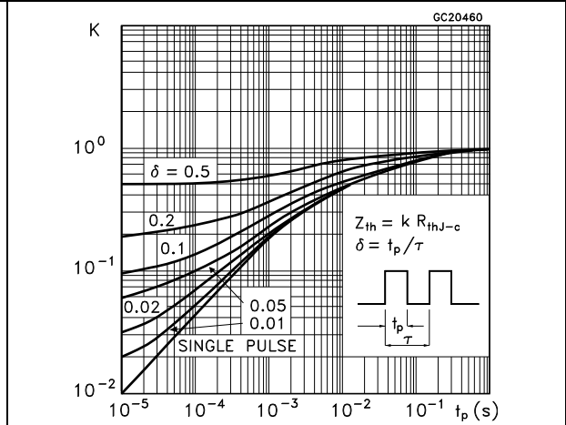
Figure 9. Thermal impedance for DPAK
