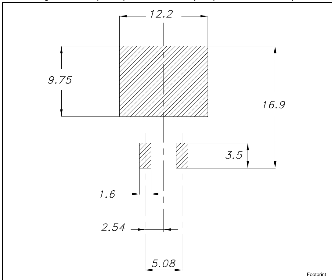
Figure 9: D 2 PAK (TO-263) recommended footprint (dimensions are in mm)
