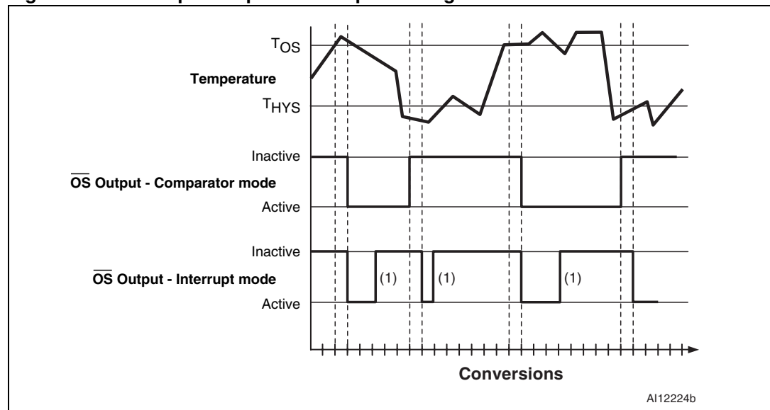
Figure 5. \overline{\text{OS}} output temperature response diagram
