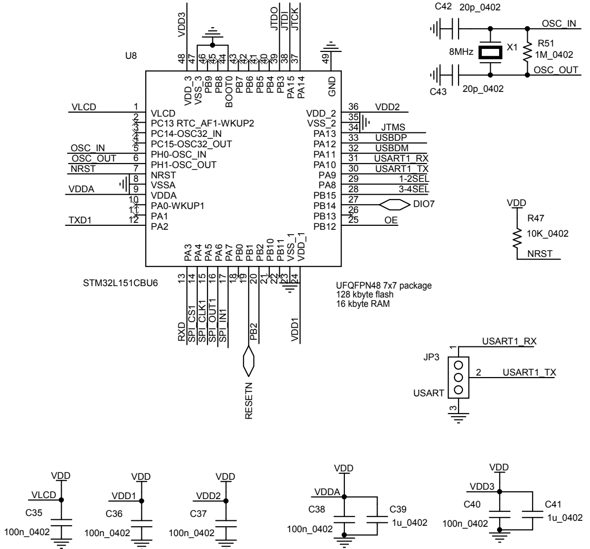
Figure 52. STEVAL-IDB008V2 - micro
