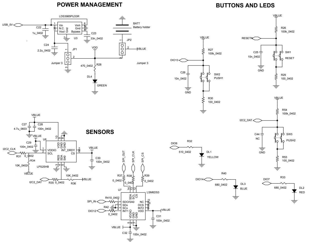
Figure 45. STEVAL-IDB007V2 - scheme 3
