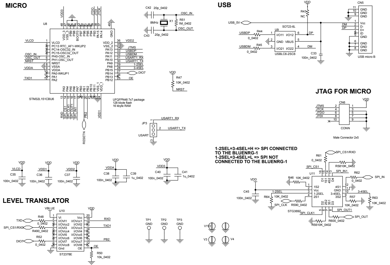
Figure 44. STEVAL-IDB007V2 - scheme 2
