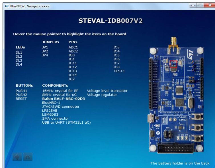
Figure 17. STEVAL-IDB007V2 kit components
