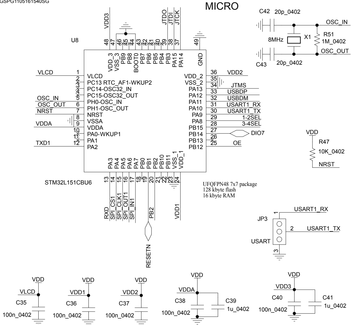
Figure 28. STEVAL-IDB007V1 micro
