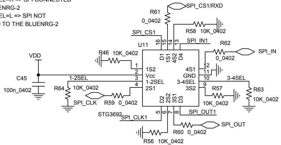
Figure 40. STEVAL-IDB008V1 switch
