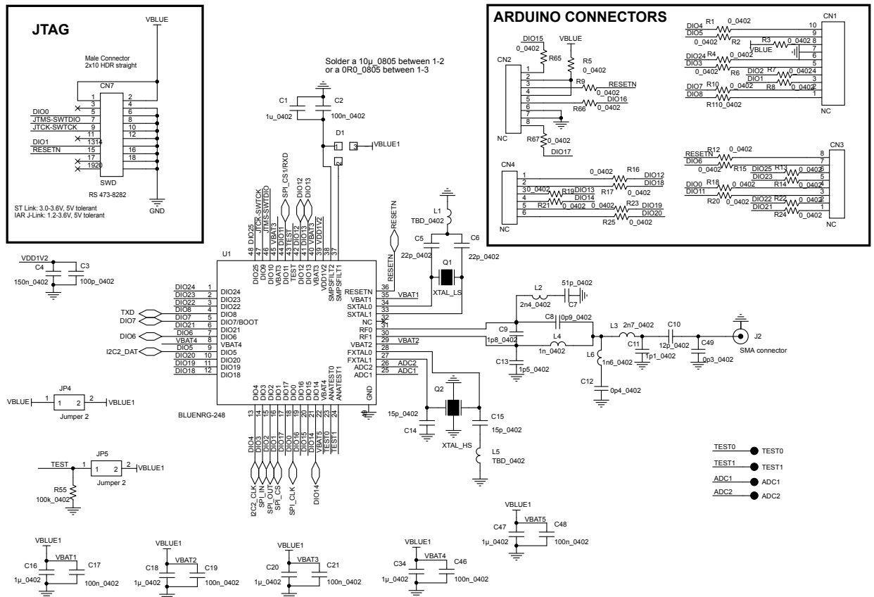
Figure 57. STEVAL-IDB009V1 schematic (1 of 3)
