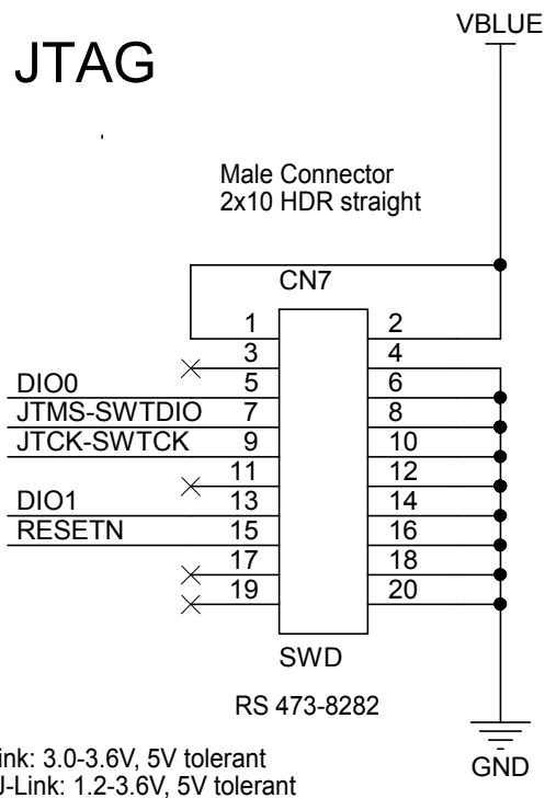
Figure 31. STEVAL-IDB008V1 circuit schematic JTAG
