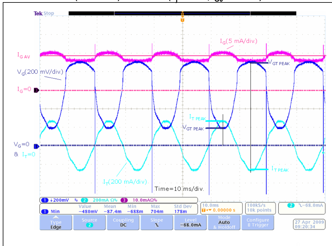
Figure 6. Example of V_{GT} variation with load current in quadrants 2 and 3 (0.2 A RMS) for a Z0103 ( T_j = 85\text{ }^\circ\text{C} , I_{G0} = 7.5\text{ mA} )
