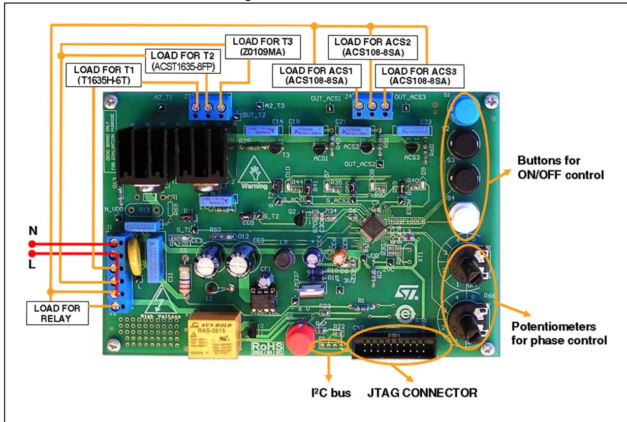
Figure 2. Board connector
