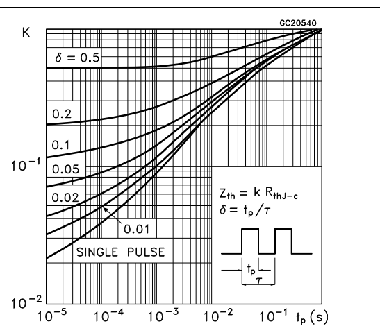
Figure 5. Thermal impedance for TO-220 and D 2 PAK
