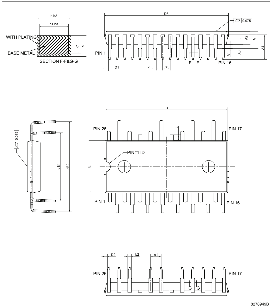
Figure 9. NDIP-26L drawing
