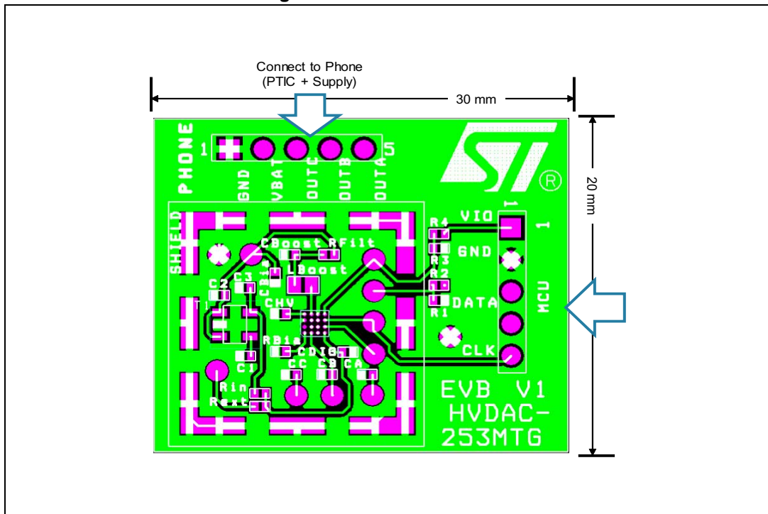
Figure 16. Evaluation board
