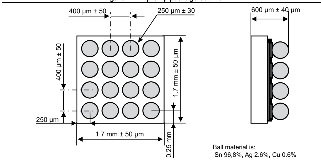
Figure 18. Footprint
