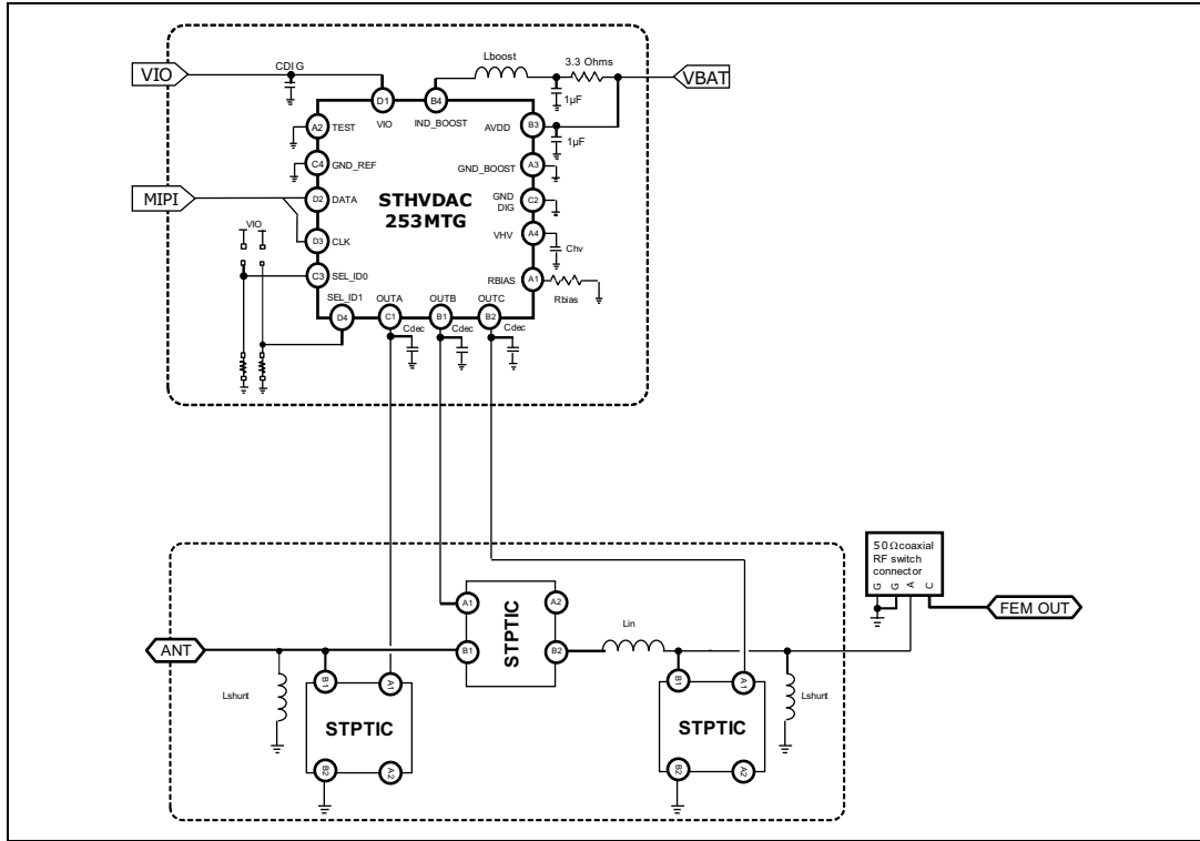
Figure 16. Evaluation board
