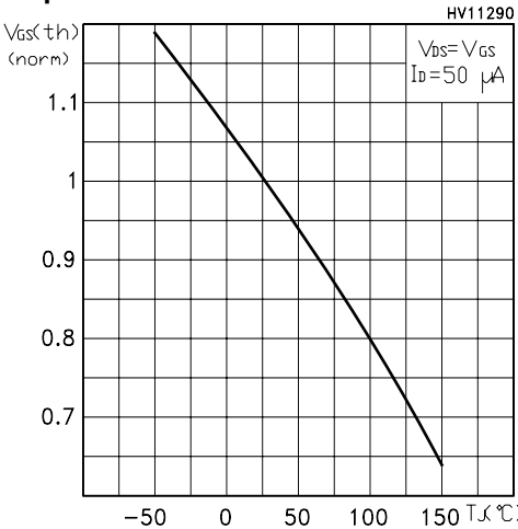
Figure 11: Normalized Gate Threshold Voltage vs Temperature
