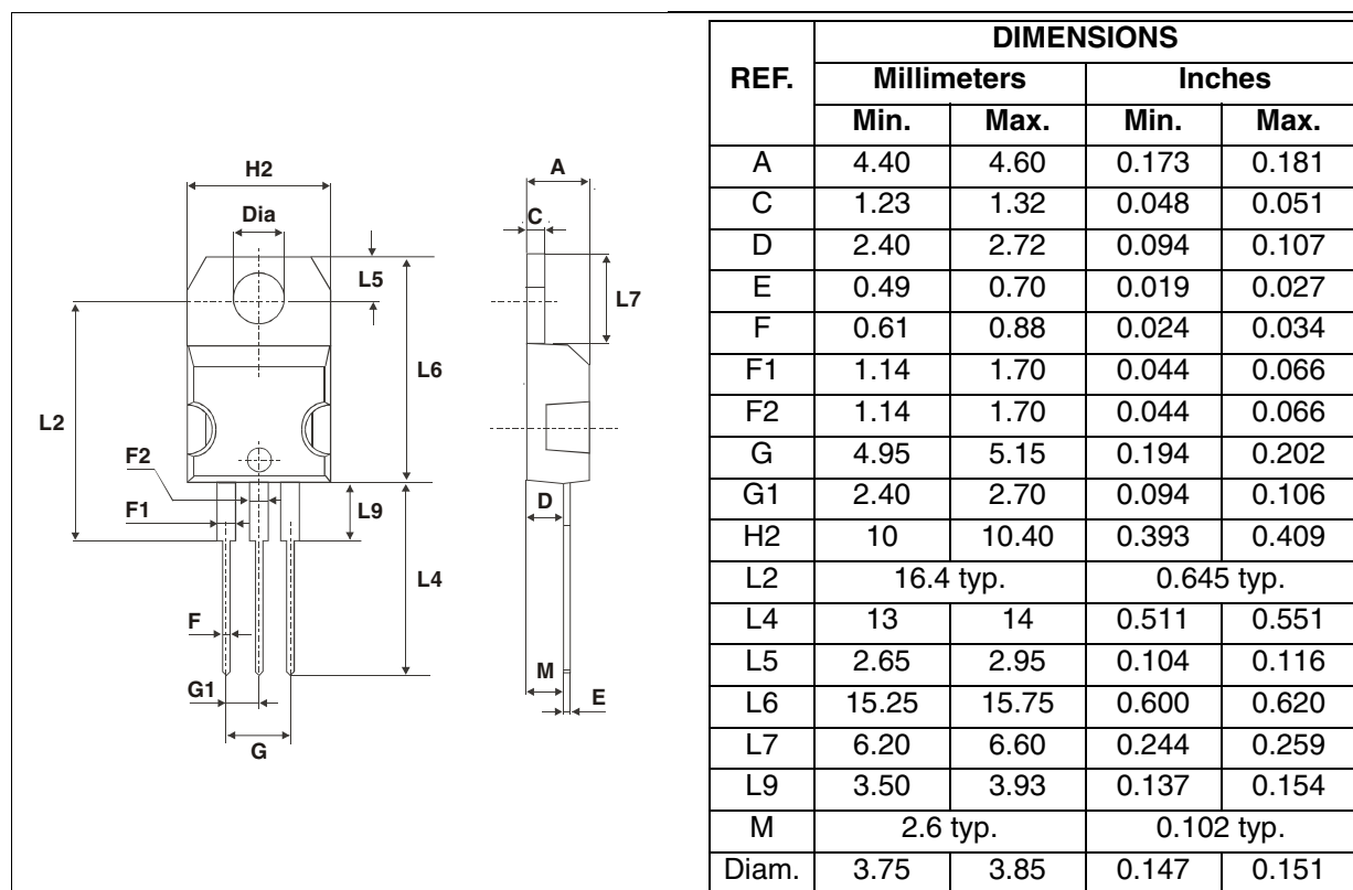
Figure 11: TO-220AB Package Mechanical Data
