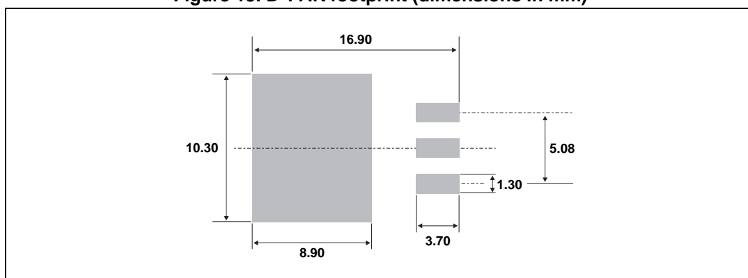
Figure 13. D 2 PAK footprint (dimensions in mm)
