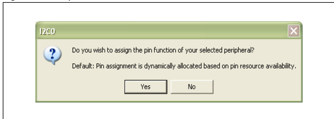
Figure 12. Prompt window
