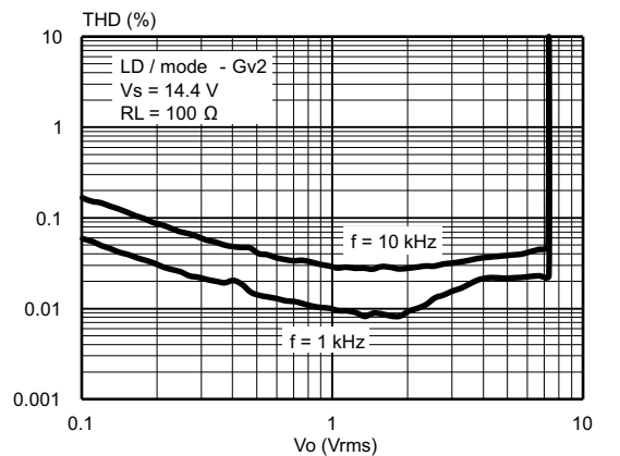
Figure 18. Distortion vs. output voltage (LD-Gv2)
