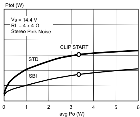
Figure 28. Power dissipation vs. average P_o (audio program simulation, 4 \Omega )
