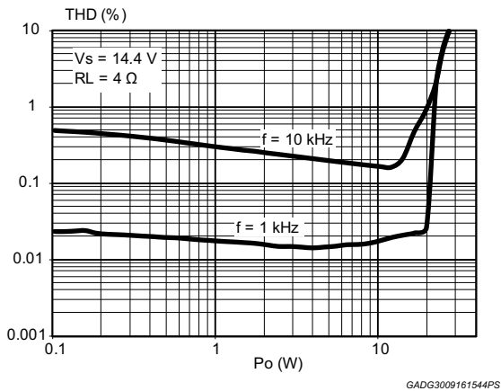
Figure 8. Distortion vs. output power (4 Ω, STD mode)
