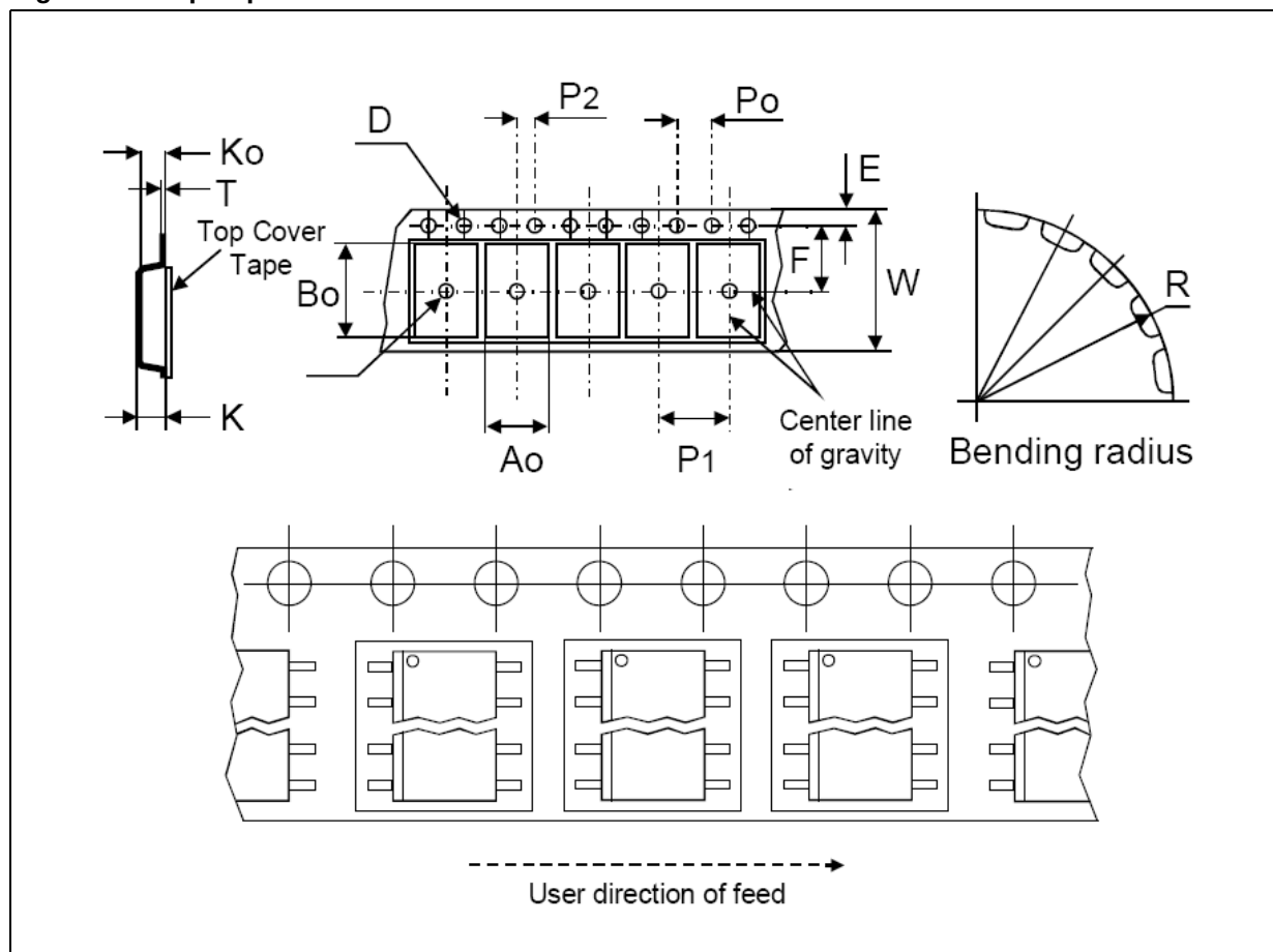
Figure 14. Tape Specification
