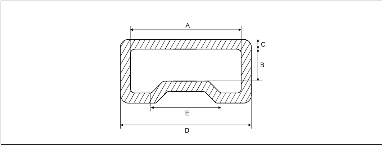
Figure 13. Tube Dimension
