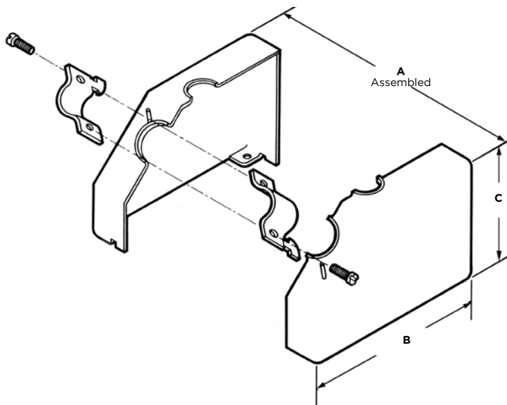
45° Cable Exit
