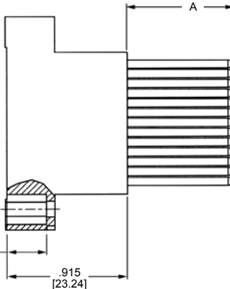
Receptacle Assembly
