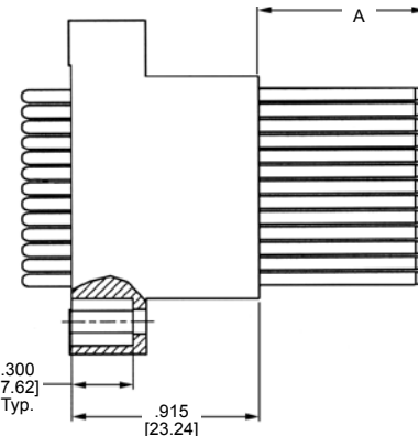
Plug Assembly
