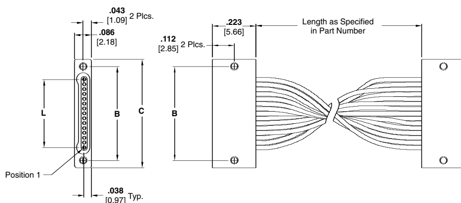
Receptacle to Receptacle Drawing Number 1589803
