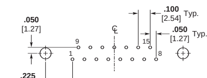
15 Contacts
