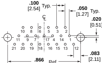
21 Contacts
