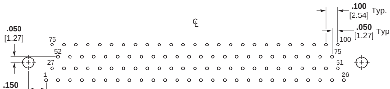
100 Contacts
