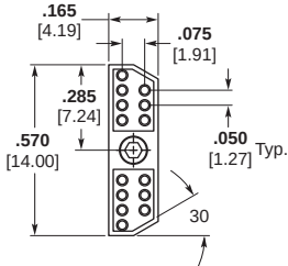
14 Layout
