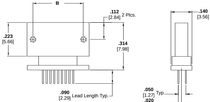
Receptacle Assembly Drawing Number 1589470
