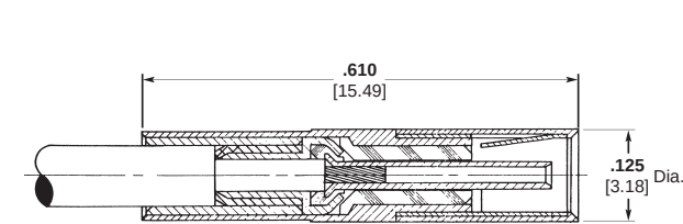
Straight Plug 1 Part Number 142-1000-0001 Instruction Sheet Number 408-08512 Former MICRODOT I.S. Number RF-ASMB-15
