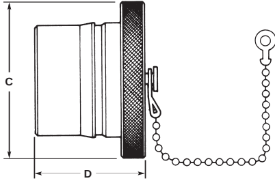
Plug Cover
