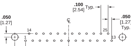
25 Contacts
