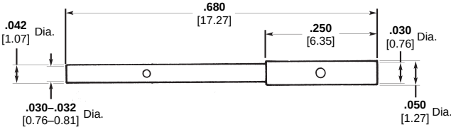
Part Number 096-0626-0001
