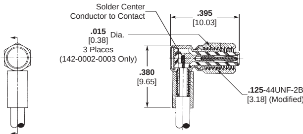
Right-Angle Plug 1
