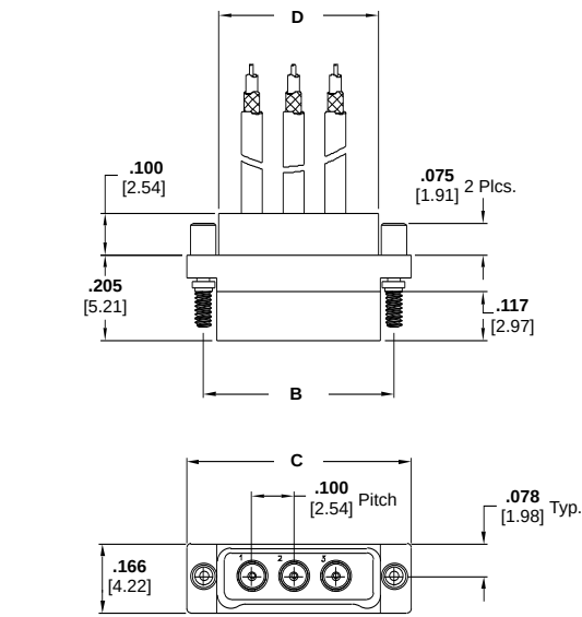
Plug Assembly Drawing Number 1589070
