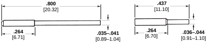
Part Number 086-0331-0000
