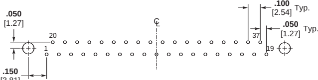
37 Contacts
