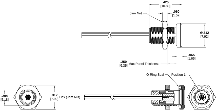
7 Position Drawing Number 1589056
