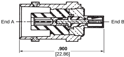
End "A" is BNC Receptacle End "B" is MICRODOT Slide-On Plug Part Number 143-1001-0001
