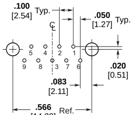
9 Contacts
