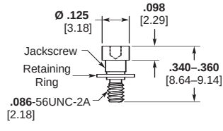
Part Number 5-1532137-5 Jackscrew Assembly Low Profile (R) 096-0002-0015 M83513/5-02 (RM) S96-0002-0087
