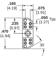
10 Layout
