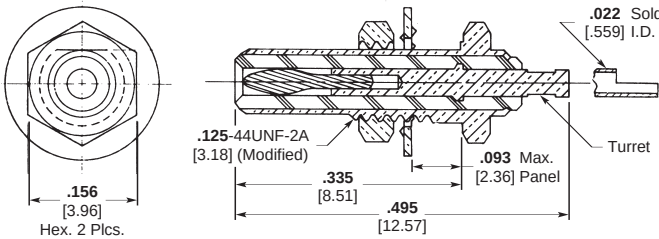
Rear Mount Receptacle
