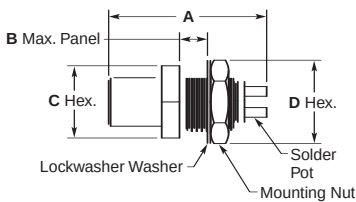
Fig. 1 Slide-On Series
