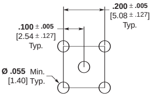
Mounting Pattern for Fig. 3 & 4
