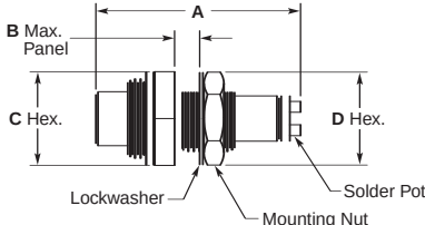
Fig. 2 Slide-On Series or Screw-On Series
