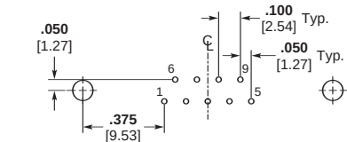
9 Contacts
