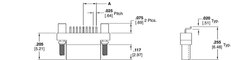
Jackscrews Omitted for Clarity
