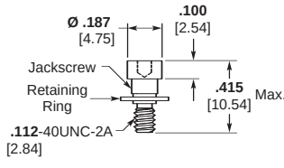
Part Number 6-1532137-0 Jackscrew Assembly Low Profile (N) 096-0002-0065 M83513/5-12 (NM) S96-0002-0091
