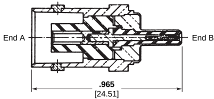
End "A" is BNC Receptacle End "B" is MICRODOT Slide-On Receptacle Part Number 143-1003-0001
