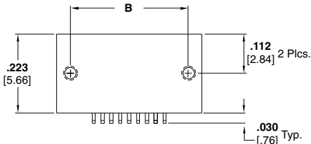
Receptacle Assembly Drawing Number 1589463
