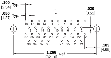
37 Contacts
