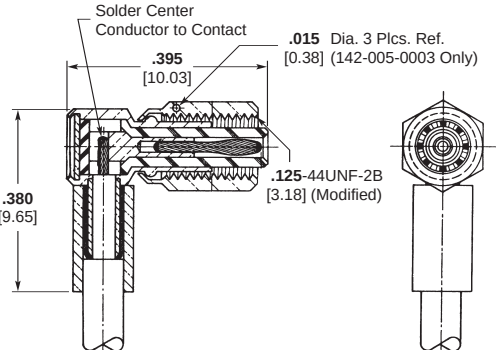
Right-Angle Plug 1
