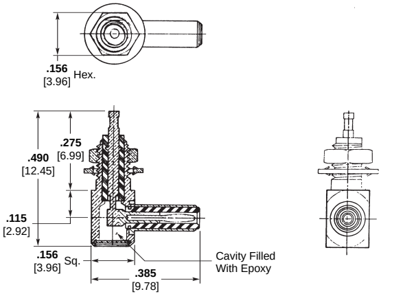
Right-Angle Receptacle Mounting Hole Shown Below Part Number 141-1012-0001
