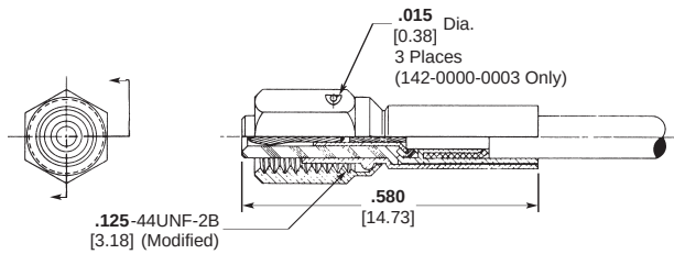
Straight Plugs 1
