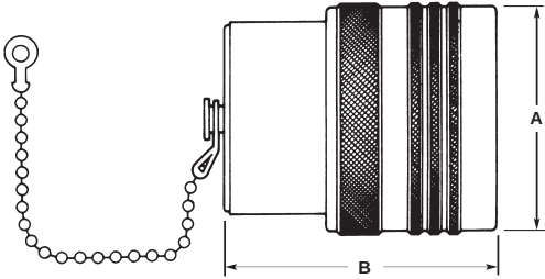
Receptacle Cover
