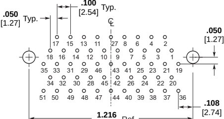
51 Contacts
