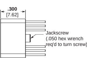
Plug
