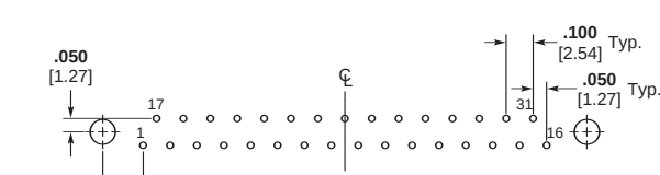
31 Contacts
