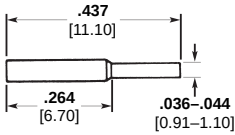
Part Number 086-0330-0000
