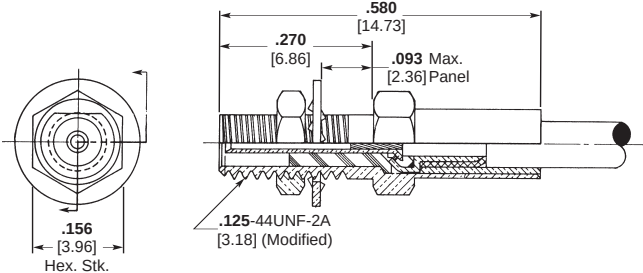
Bulkhead Jack 1
