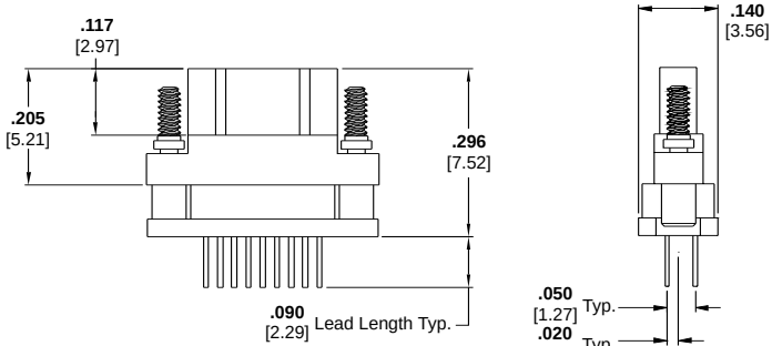
Plug Assembly Drawing Number 1589461
