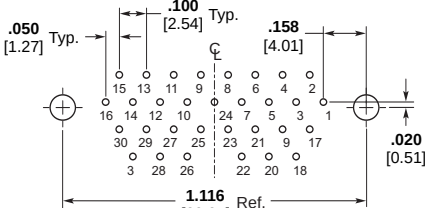
31 Contacts
