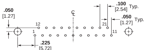
21 Contacts
