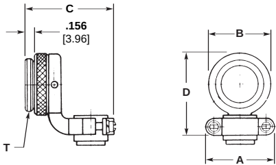
Right-Angle
