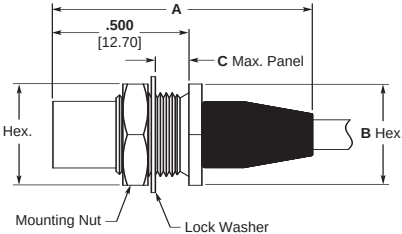
Fig. 3 Bulkhead Plug
