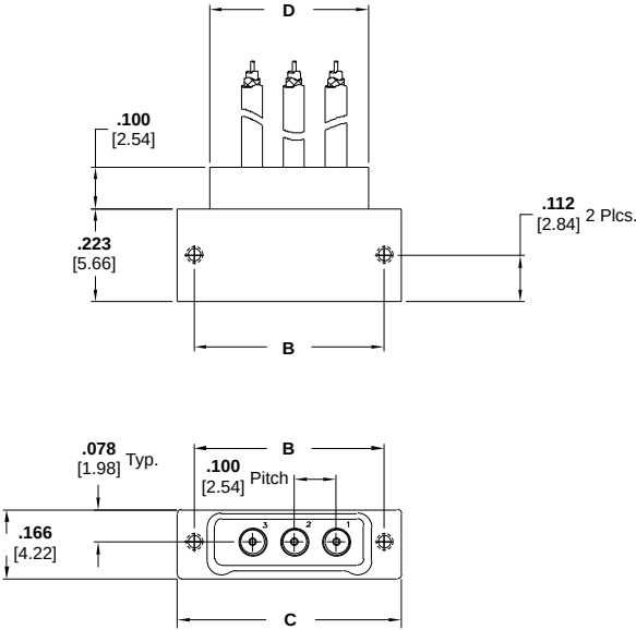
Receptacle Assembly Drawing Number 1589071
