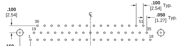
51 Contacts
