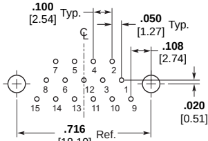
15 Contacts
