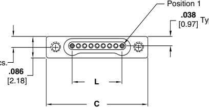
Receptacle with Flying Leads Drawing Number 1589457
