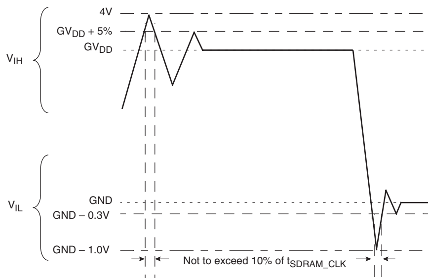
Figure 2-1. Overshoot/Undershoot Voltage
