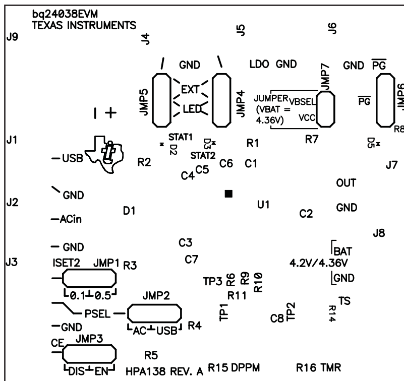
Figure 4. Board Layout – Silkscreen
