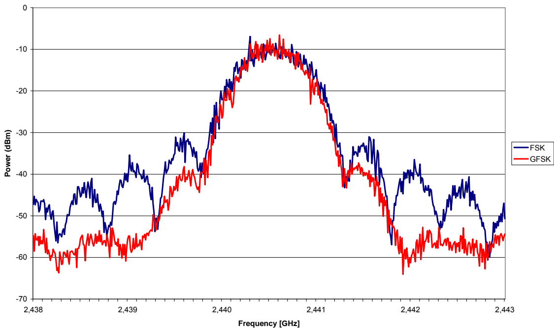
Figure 18. Modulated spectrum
