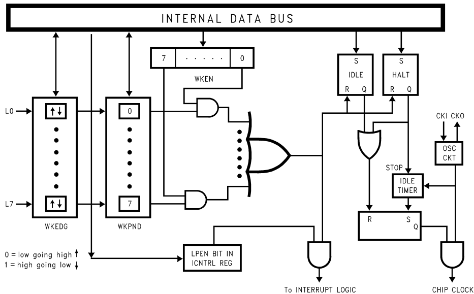
Figure 24. Multi-Input Wake-Up Logic
