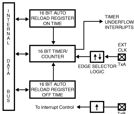
Figure 20. Timer in External Event Counter Mode
