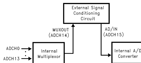
Figure 29. A/D with Single Ended Mux Output Feature Enabled
