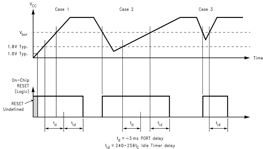
Figure 12. Brownout Reset Operation
