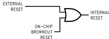
Figure 10. Reset Logic
