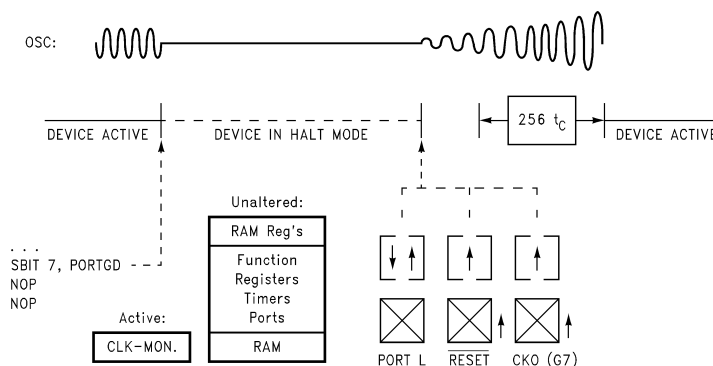
Figure 23. Wake-up from HALT
