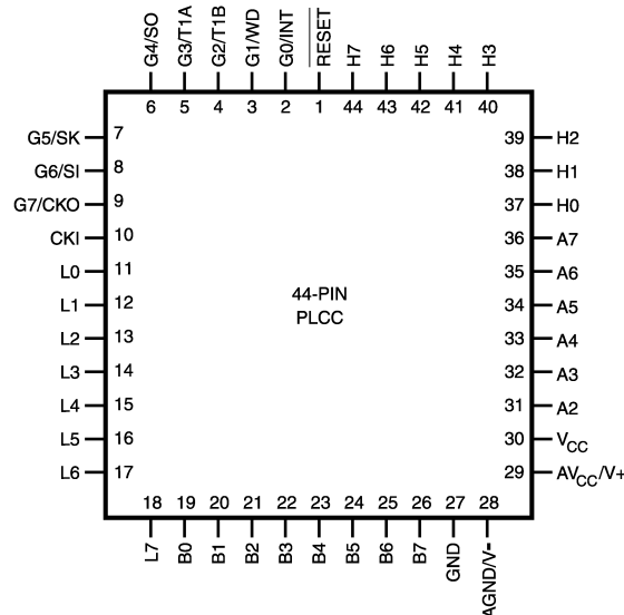
Figure 1. Top View
