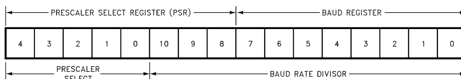
Figure 28. USART BAUD Clock Divisor Registers
