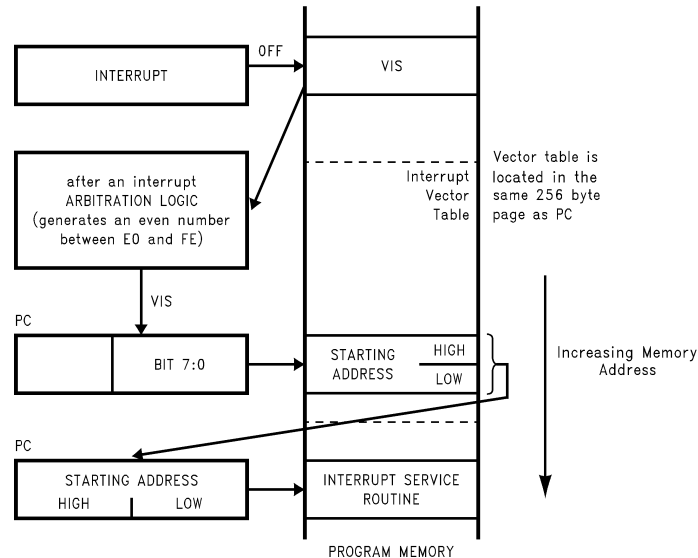
Figure 33. VIS Operation
