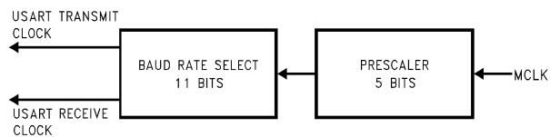
Figure 27. USART BAUD Clock Generation
