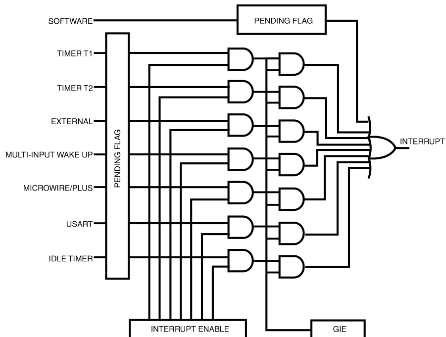
Figure 32. Interrupt Block Diagram
