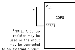
Figure 13. Reset Circuit Using Power-On Reset
