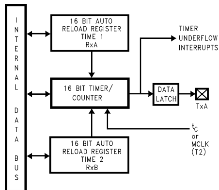
Figure 19. Timer in PWM Mode
