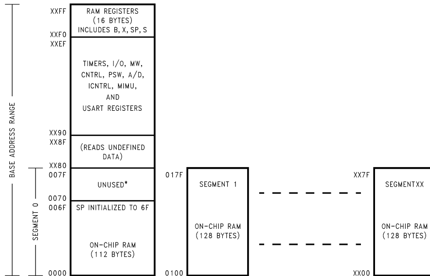
Figure 9. RAM Organization
