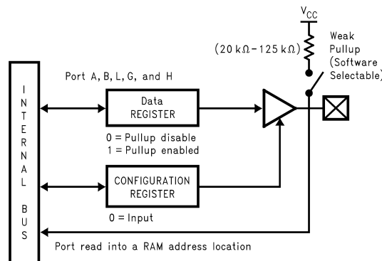
Figure 7. I/O Port Configurations—Input Mode
