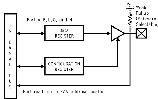
Figure 5. I/O Port Configurations
