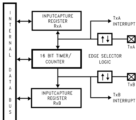
Figure 21. Timer in Input Capture Mode
