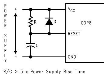
Figure 11. Reset Circuit Using External Reset
