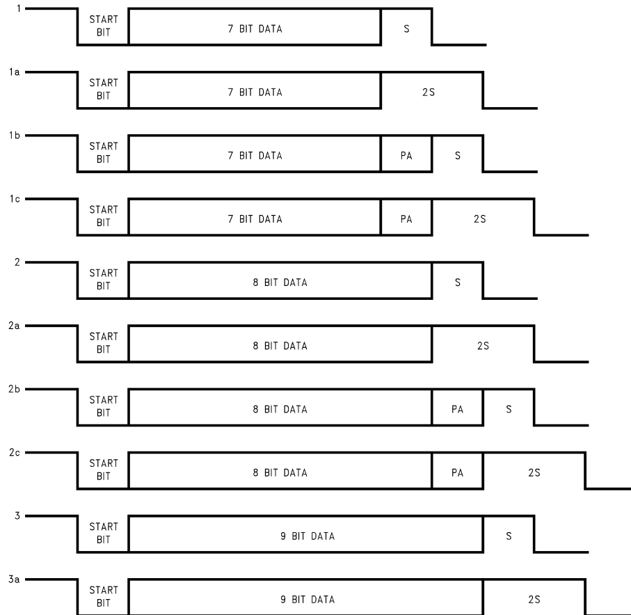
Figure 26. Framing Formats
