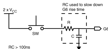
Figure 17. Circuit Diagram for Implementing the 2 \times V_{CC}
