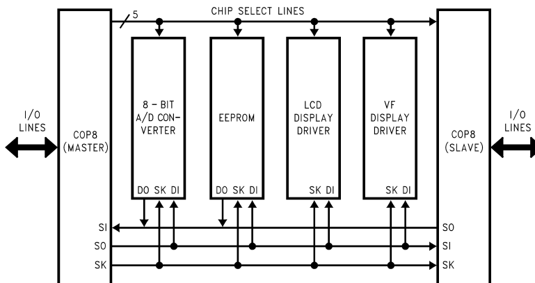
Figure 35. MICROWIRE/PLUS Application
