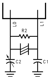
Figure 15. Low Speed Oscillator
