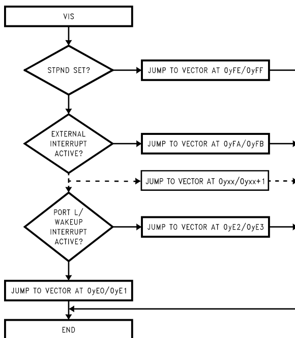
Figure 34. VIS Flow Chart
