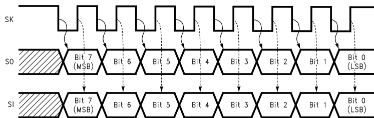
Figure 39. MICROWIRE/PLUS SPI Mode Interface Timing, Alternate SK Mode, SK Idle Phase being High
