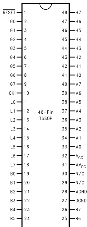
Figure 3. Top View
