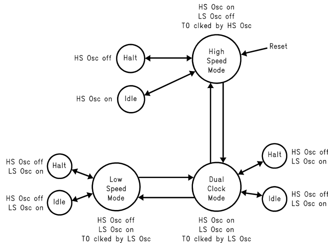
Figure 22. Diagram of Power Save Modes
