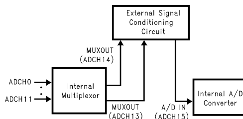
Figure 30. A/D with Differential Mux Output Feature Enabled
