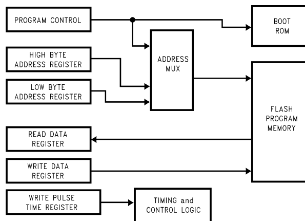
Figure 16. Block Diagram of ISP
