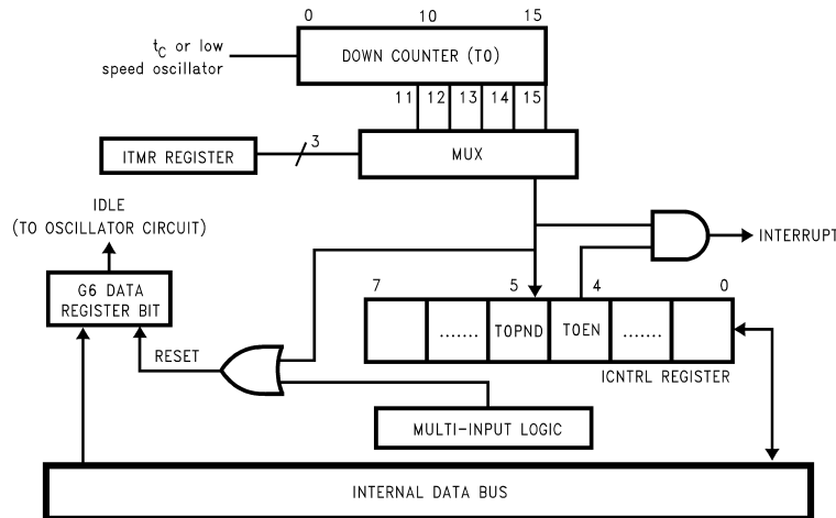
Figure 18. Functional Block Diagram for Idle Timer T0
