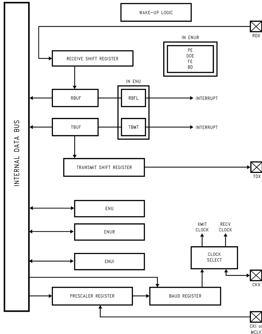
Figure 25. USART Block Diagram
