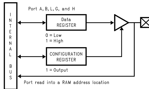
Figure 6. I/O Port Configurations—Output Mode
