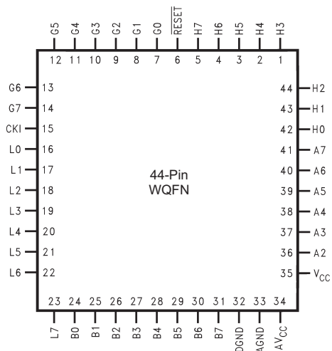
Figure 2. Top View
