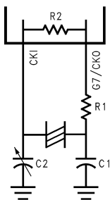
Figure 14. High Speed Oscillator
