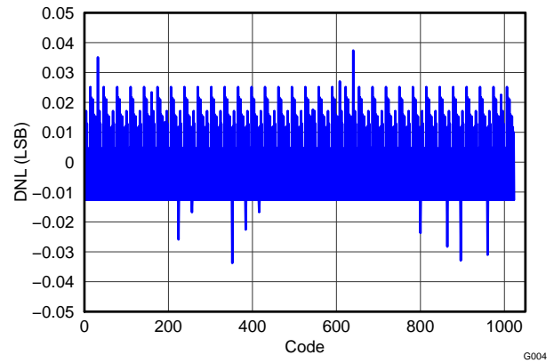
Figure 6. DAC3151 Differential Nonlinearity
