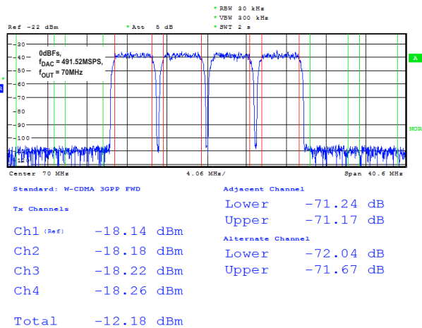
Figure 61. DAC3171 Four-Carrier WCDMA Test Mode 1
