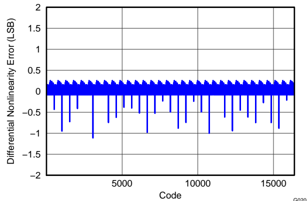
Figure 46. DAC3171 Differential Nonlinearity
