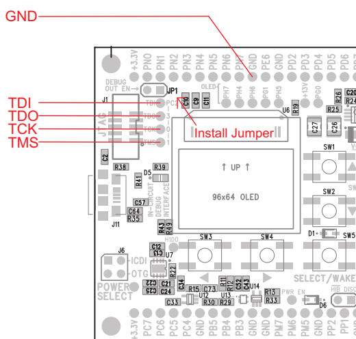
Figure 2-3. Debug Out
