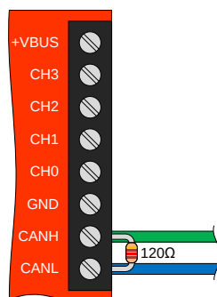
Figure 2-2. Can Diagram
