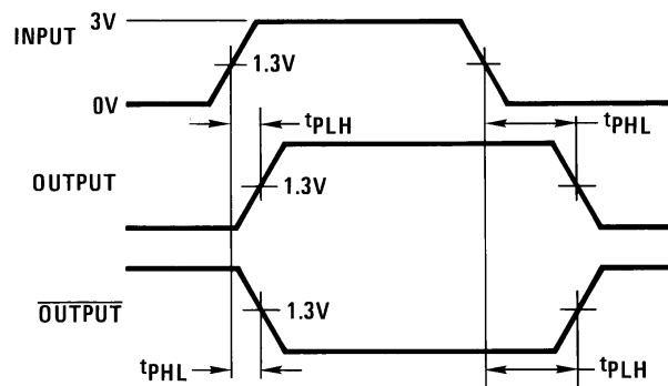
Figure 3. Propagation Delays
