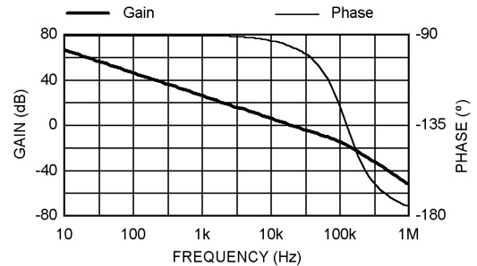
FIGURE 13. Example Loop Transfer Function
