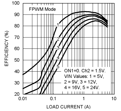
Efficiency vs Load Current (Ch2, Typical Application, FPWM = 0)
