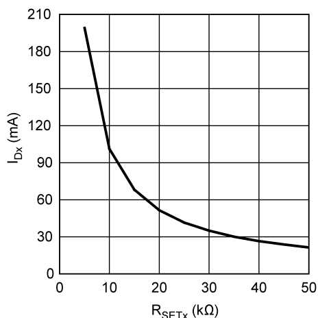
Dx Current vs. R_{SET}
