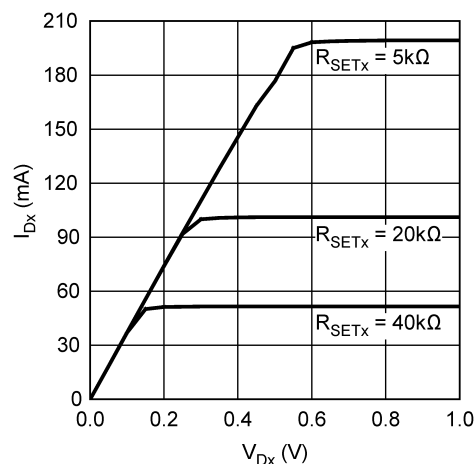
Dx Current vs. Headroom Voltage
