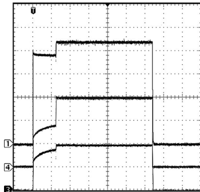
Startup and Shutdown Response Torch Mode (400mA)
