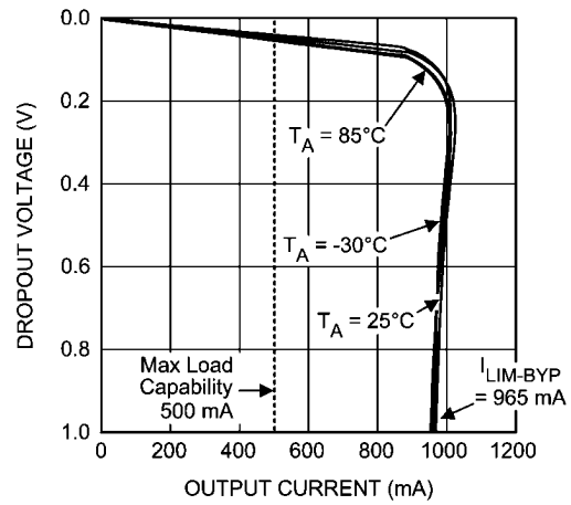
Dropout Voltage vs Output Current (Bypass mode, V_{IN} = 3.6V )
