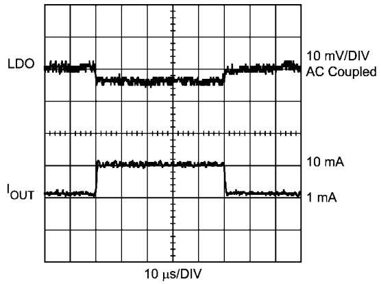
LDO Load Transient Response (C OUT = 1μF)
