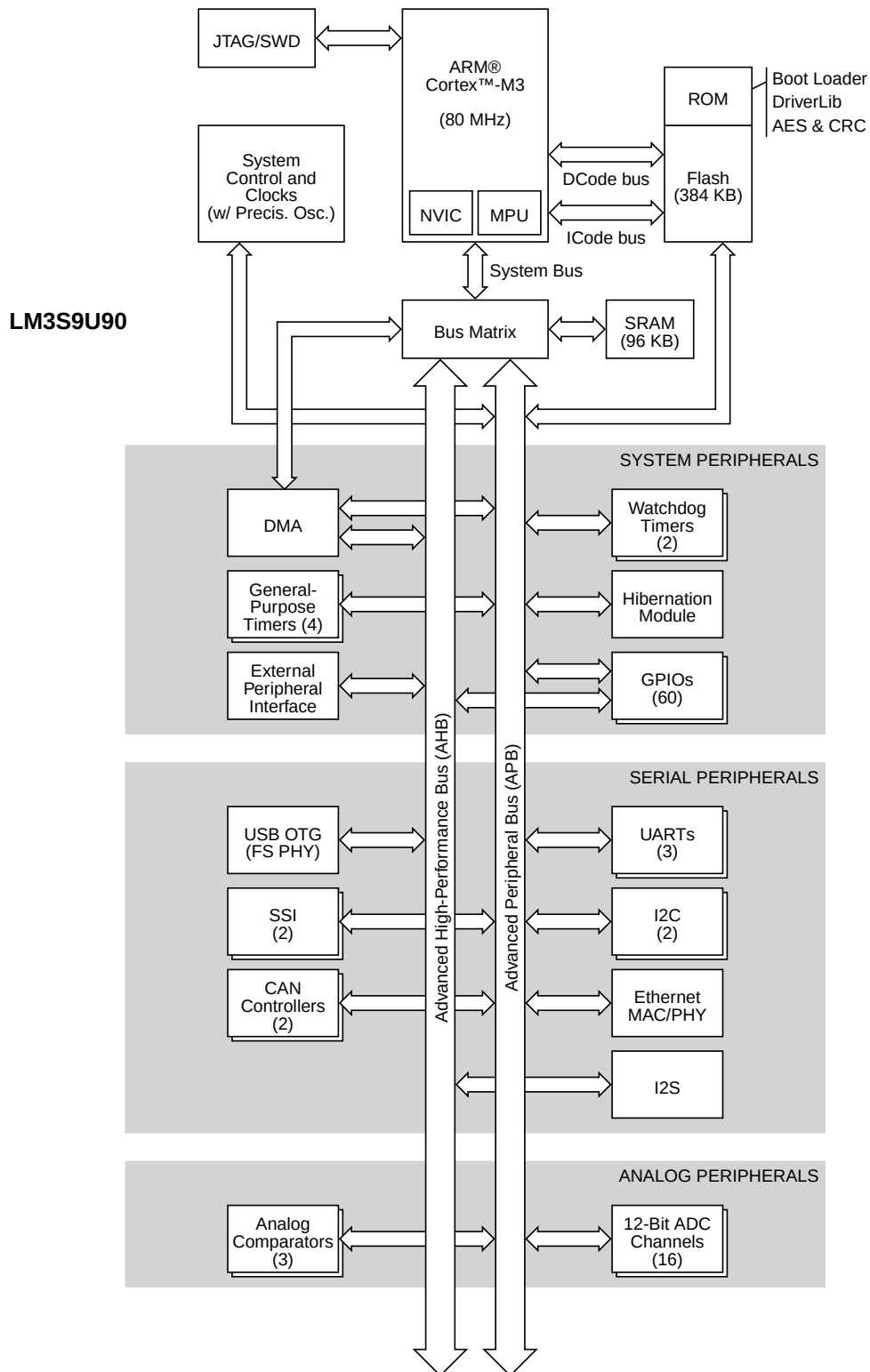
Figure 1-1. Stellaris LM3S9U90 Microcontroller High-Level Block Diagram
