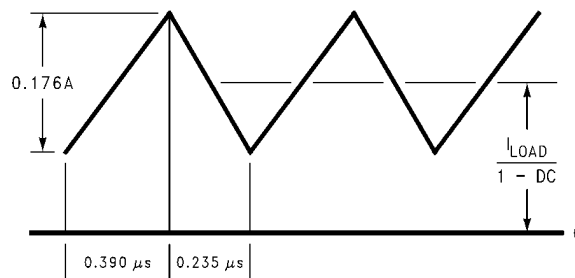
FIGURE 2. 10 \mu\text{H} Inductor Current 5V - 12V Boost (LM4960)
