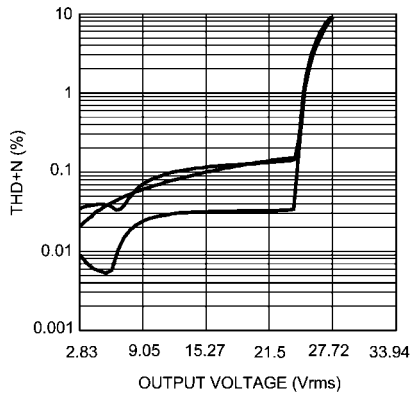
THD+N vs Output Power V_{DD} = 5V, V_1 = 12V, f = 100\text{Hz}, 1\text{kHz}, 10\text{kHz}
