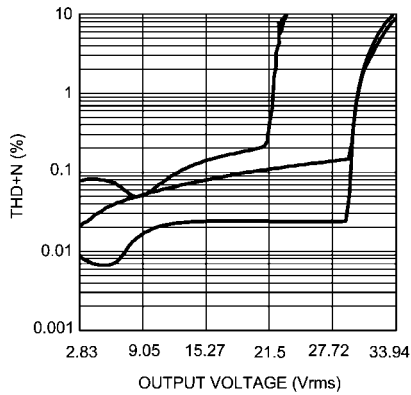
THD+N vs Output Power V_{DD} = 3V, V_1 = 15V, f = 100\text{Hz}, 1\text{kHz}, 10\text{kHz}
