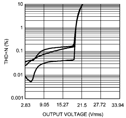
THD+N vs Output Power V_{DD} = 5V, V_1 = 9.6V, f = 100\text{Hz}, 1\text{kHz}, 10\text{kHz}
