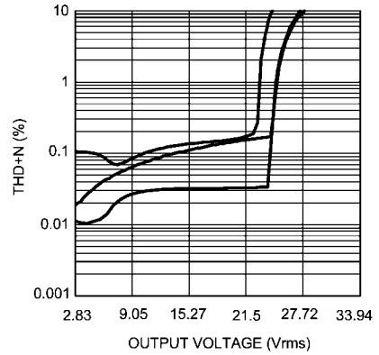
THD+N vs Output Power V_{DD} = 3V, V_1 = 12V, f = 100\text{Hz}, 1\text{kHz}, 10\text{kHz}
