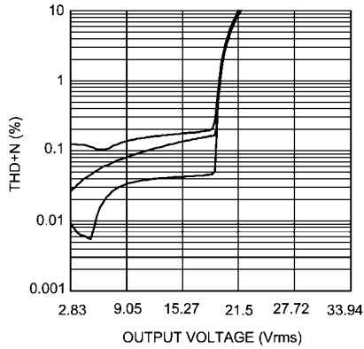
THD+N vs Output Power V_{DD} = 3V, V_1 = 9.6V, f = 100\text{Hz}, 1\text{kHz}, 10\text{kHz}
