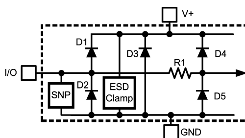
FIGURE 4. ESD Protection Input Structure. Devices that are connected to a particular pin are marked with a "✓" in the table above.
