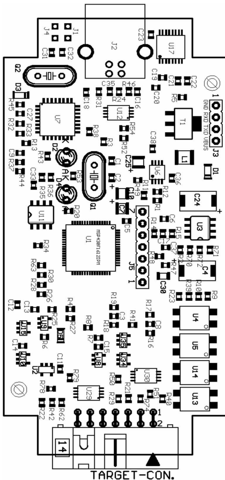
Figure B-47. MSP-FET430UIF USB Interface, PCB
