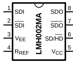
Figure 1. 8-Pin SOIC See D Package
