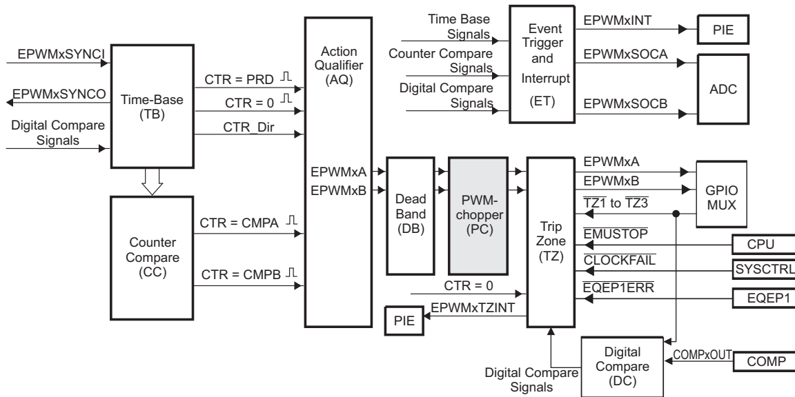
Figure 3-33. PWM-Chopper Submodule
