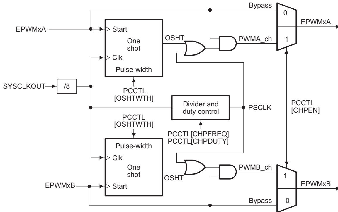
Figure 3-34. PWM-Chopper Submodule Operational Details
