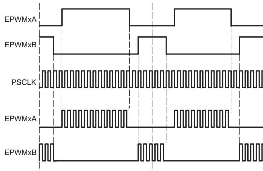
Figure 3-35. Simple PWM-Chopper Submodule Waveforms Showing Chopping Action Only
