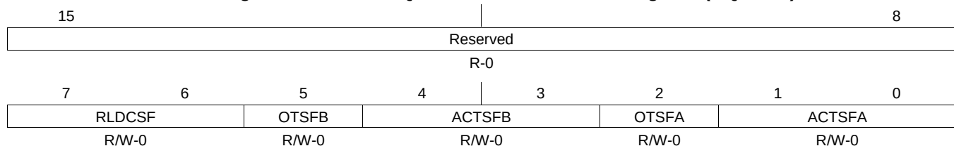
Figure 3-92. Action-Qualifier Software Force Register (AQSFRC)
