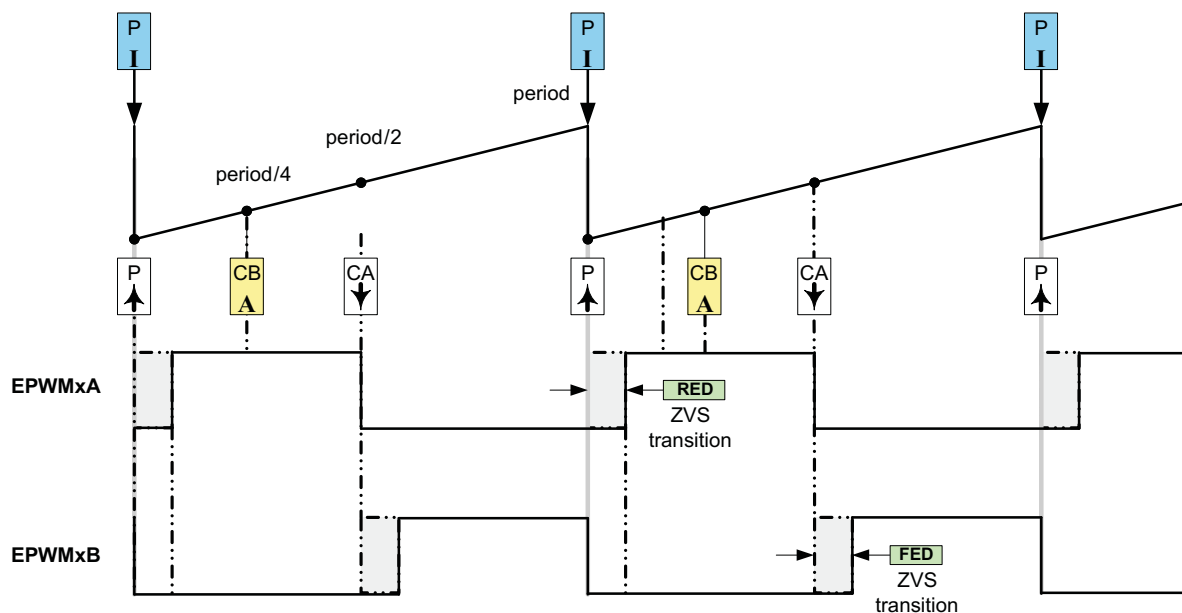
Figure 3-73. H-Bridge LLC Resonant Converter PWM Waveforms
