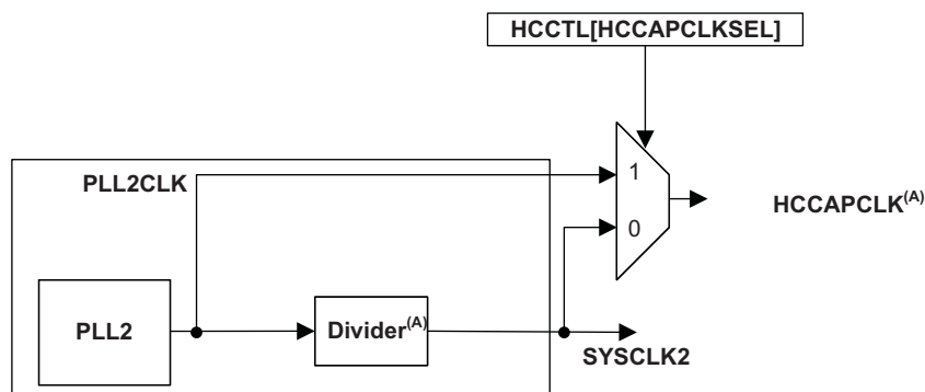
Figure 5-3. HCCAPCLK Generation
