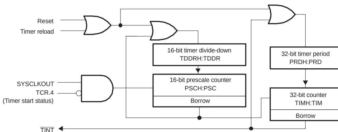
Figure 1-43. CPU-Timer Interrupts Signals and Output Signal
