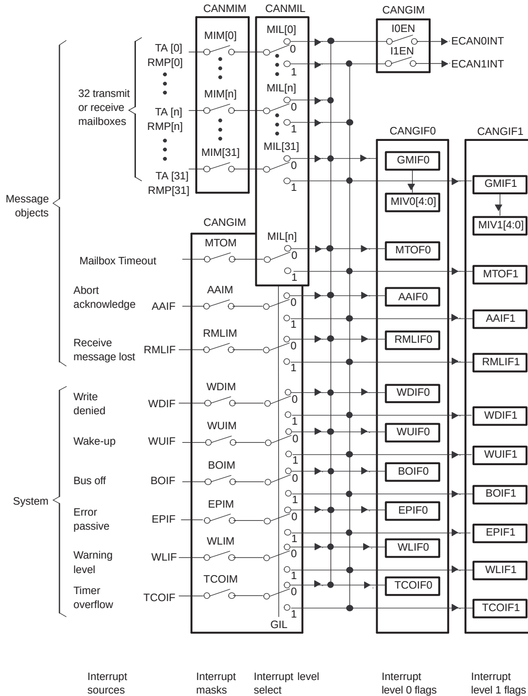
Figure 16-42. Interrupts Scheme
