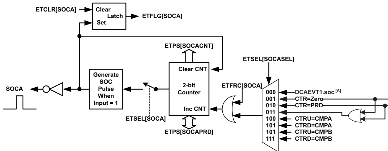
Figure 3-45. Event-Trigger SOCA Pulse Generator
