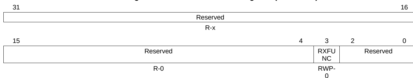
Figure 16-27. RX I/O Control Register (CANRIOC)
