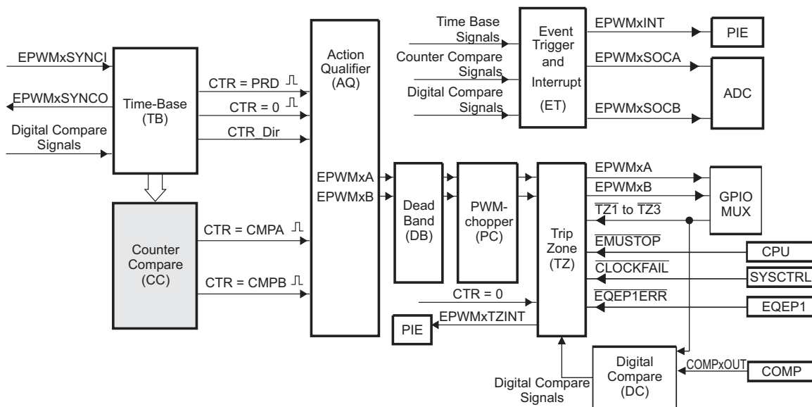
Figure 3-14. Counter-Compare Submodule
