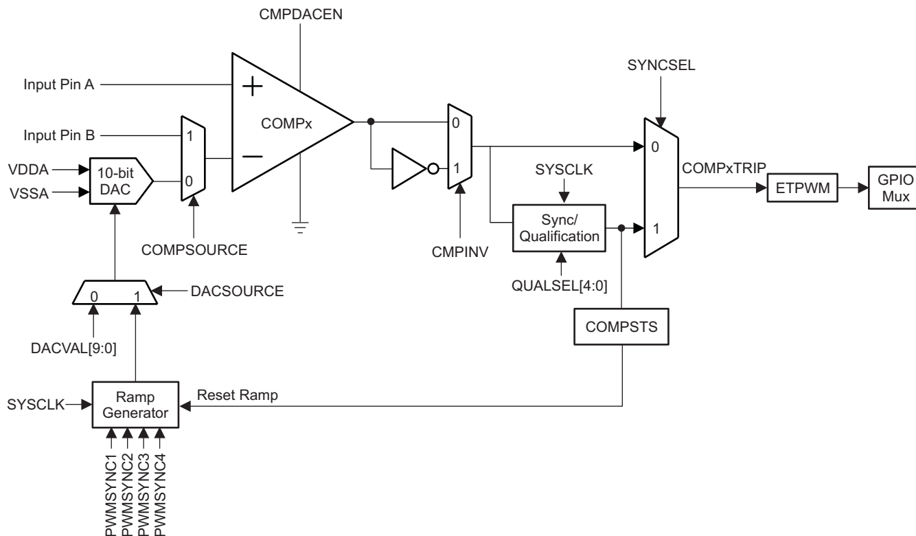
Figure 8-39. Comparator Block Diagram
