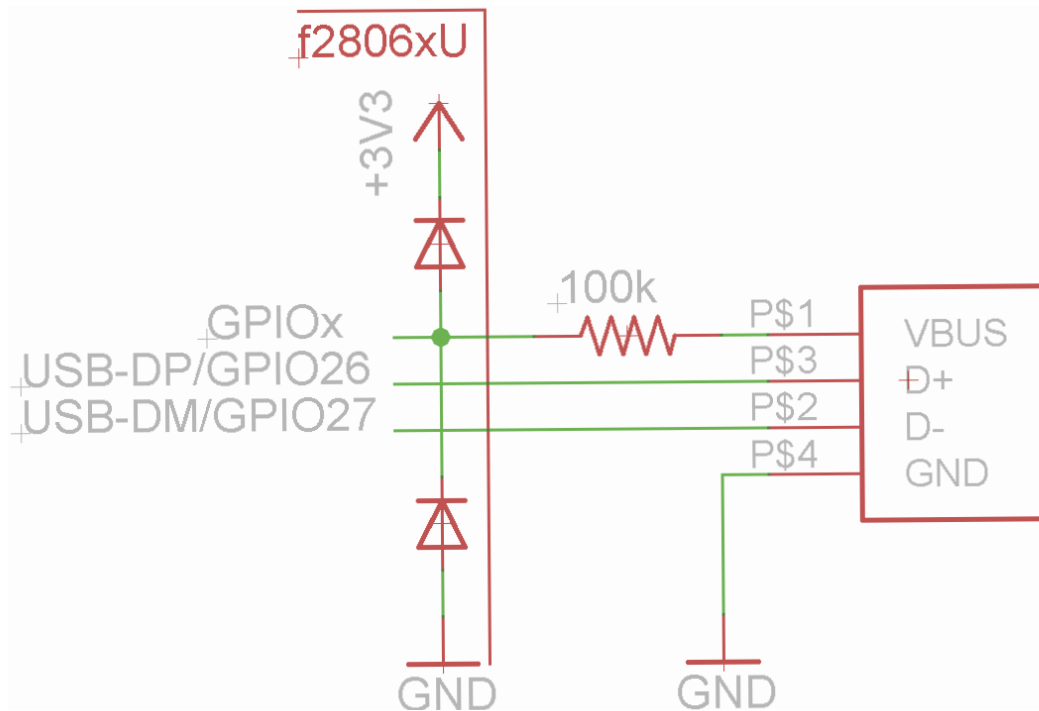
Figure 17-2. USB Scheme
