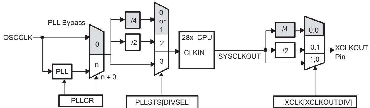
Figure 1-35. XCLKOUT Generation
