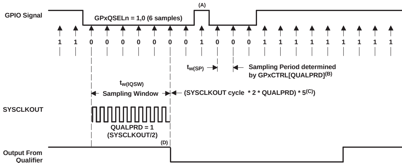
Figure 1-57. Input Qualifier Clock Cycles
