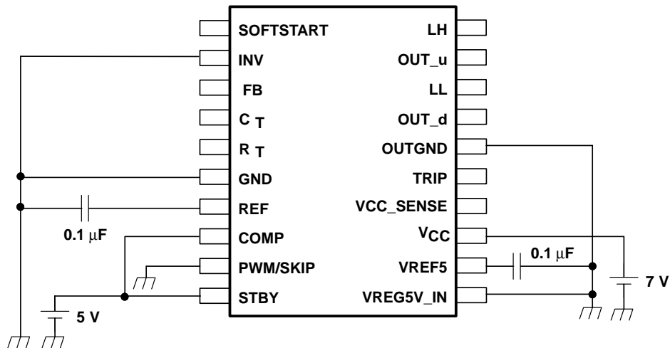
Figure 2. Test Circuit
