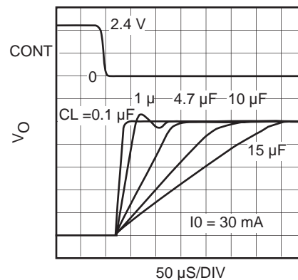
CONTROL RESPONSE (OFF → ON)
