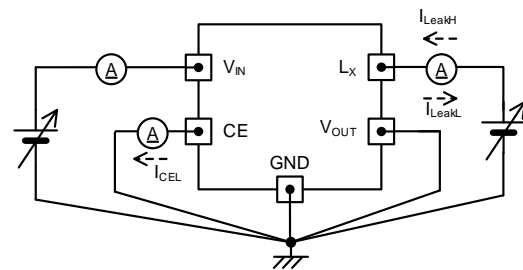
< Circuit No.⑥ >
