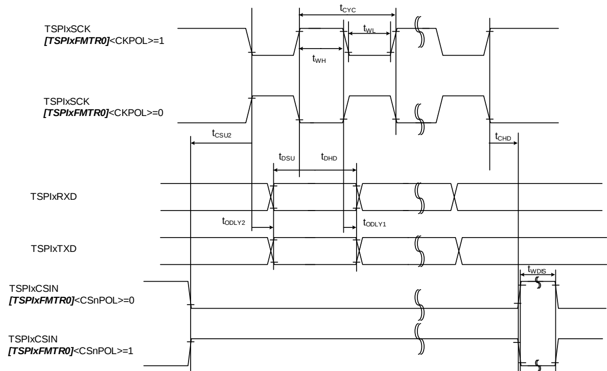
Figure 7.3 2 nd clock edge sampling (Slave)
