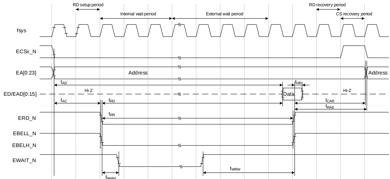
Figure 7.8 Read cycle timing (external wait)
