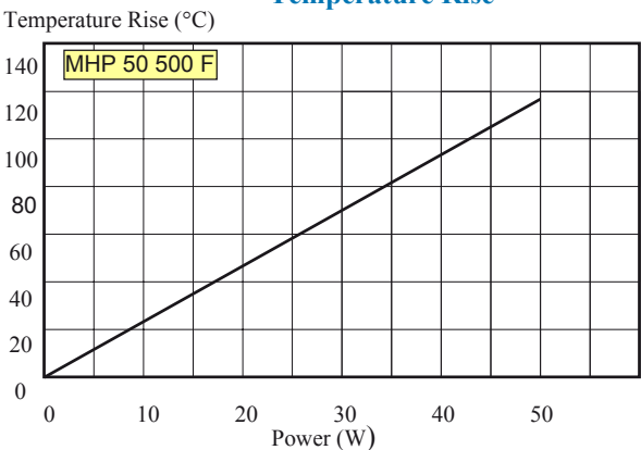
Temperature Rise
