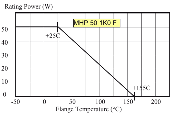
Derating
