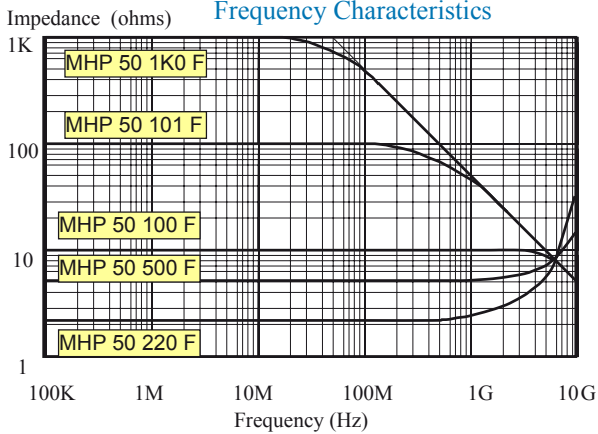
Frequency Characteristics
