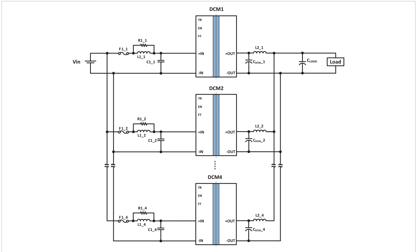
Typical Application 1: DCM48AP150x320A50 in an array of four units
