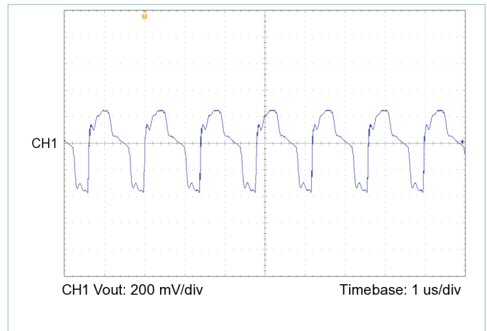
Figure 19 — Output voltage ripple, V_{IN} = 48\text{ V} , V_{OUT} = 15.0\text{ V} , C_{OUT\_EXT} = 1000\text{ }\mu\text{F} , R_{LOAD} = 0.701\text{ }\Omega
