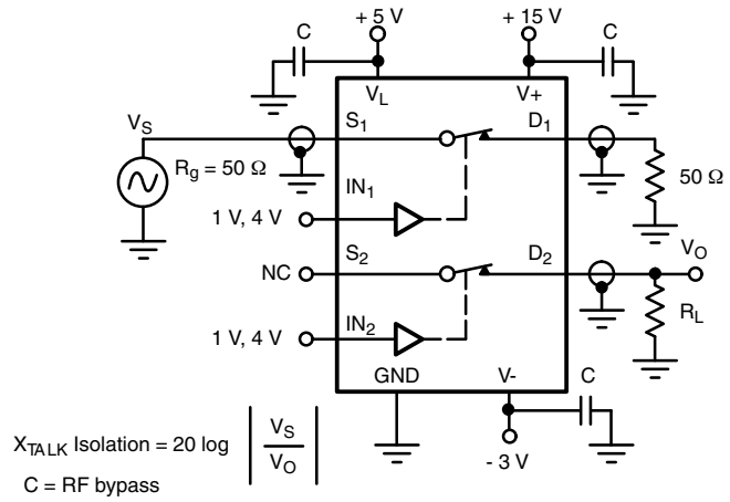
Figure 4. Crosstalk
