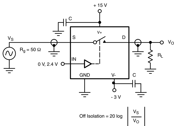
Figure 4. Off Isolation
