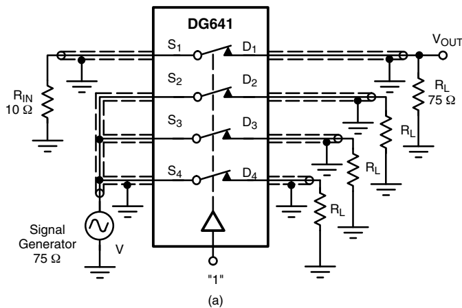
Figure 5. All Hostile Crosstalk - X_{TALK(AH)}
