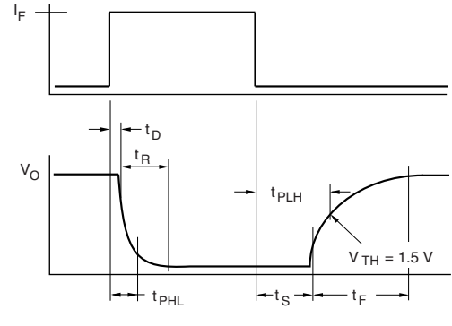
Fig. 6 - Saturated Switching Timing
