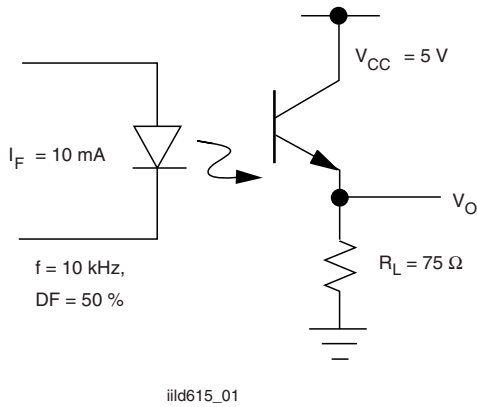
Fig. 3 - Non-Saturated Switching Timing
