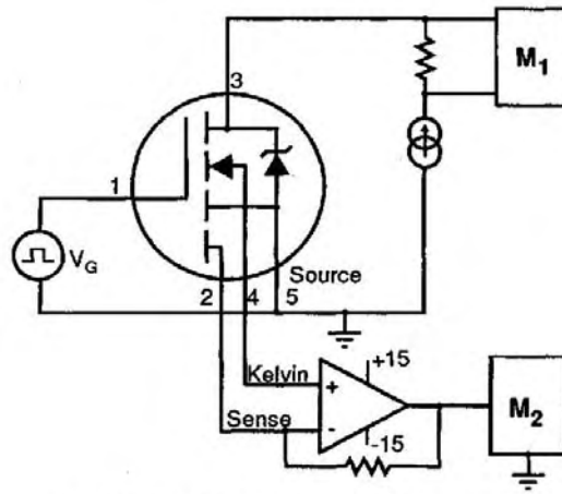
Fig 18. HEXSense Ratio Test Circuit
