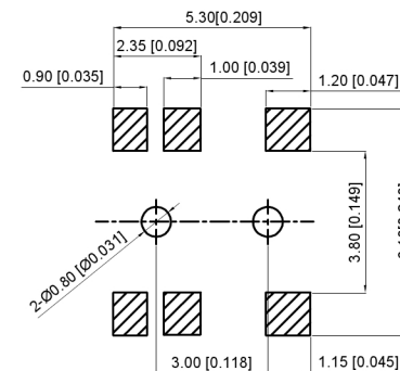
PCB Installation Dimension Drawing PCB安装尺寸图
