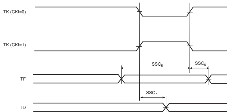
Figure 57-30. SSC Transmitter, TK and TF in Input
