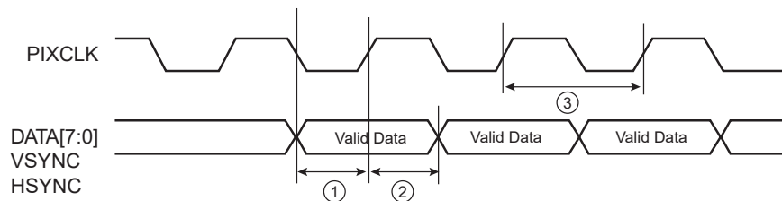
Figure 57-36. ISI Timing Diagram
