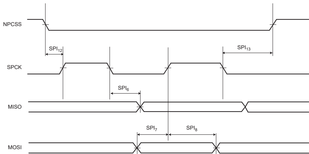
Figure 57-16. SPI Client Mode with (CPOL=0 and NCPHA=1) or (CPOL=1 and NCPHA=0)
