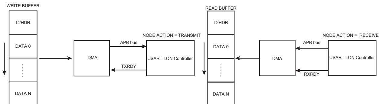
Figure 45-64. DMAM = 0
