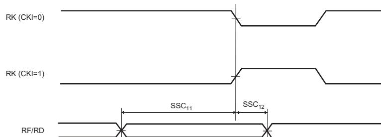
Figure 57-34. SSC Receiver, RK in Output and RF in Input
