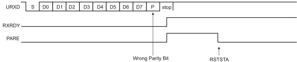
Figure 46-7. Parity Error
