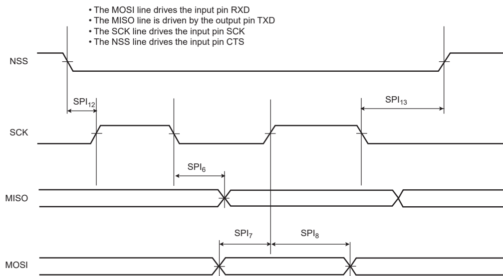
Figure 57-21. USART SPI Client Mode (Mode 1 or 2)
