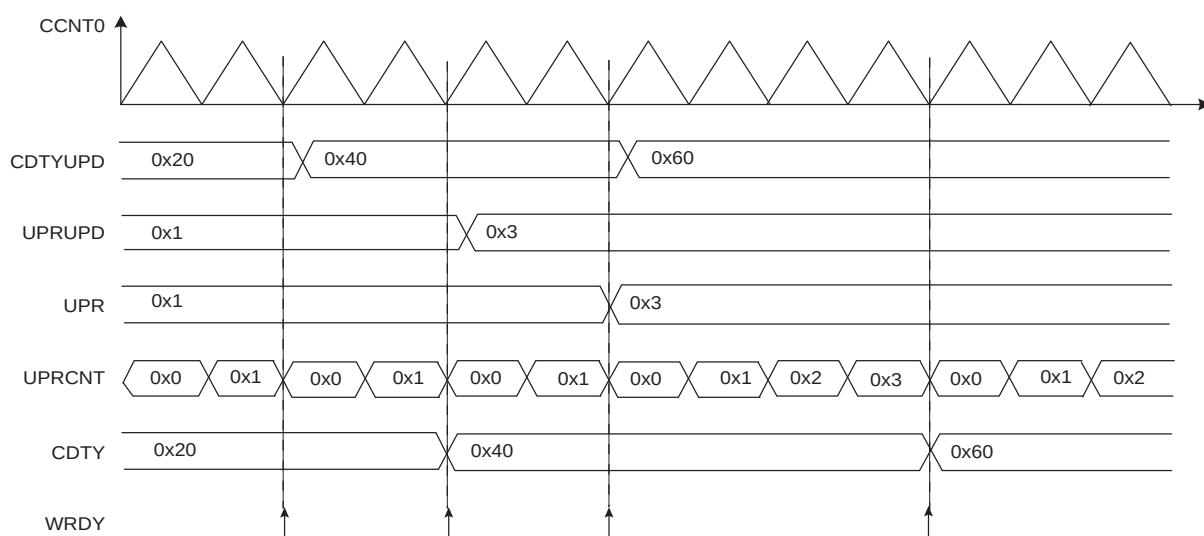
Figure 50-20. Method 2 (UPDM = 1)
