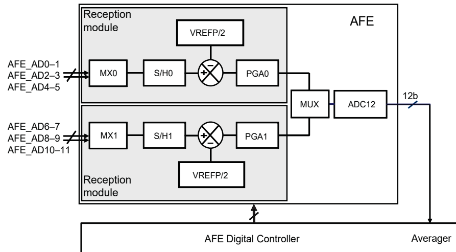
Figure 51-16. Differential Mode AFE
