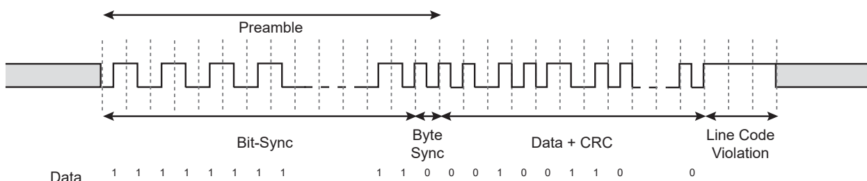
Figure 45-55. LON Framing
