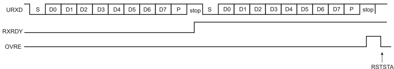
Figure 46-6. Receiver Overrun
