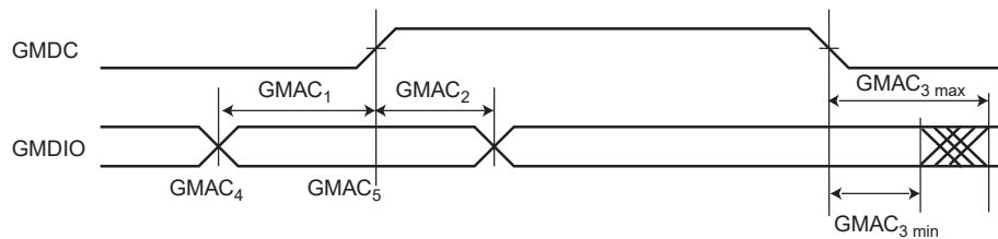
Figure 57-24. Min and Max Access Time of GMAC Output Signals
