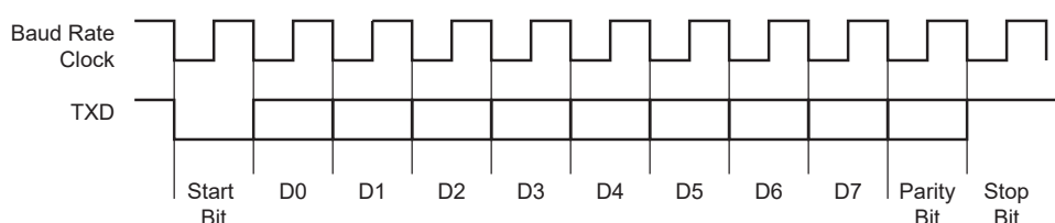
Figure 45-5. Character Transmit
