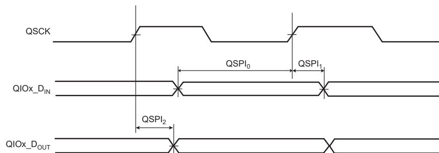
Figure 57-11. QSPI Host Mode with (CPOL = 0 and CPHA = 1) or (CPOL = 1 and CPHA = 0)
