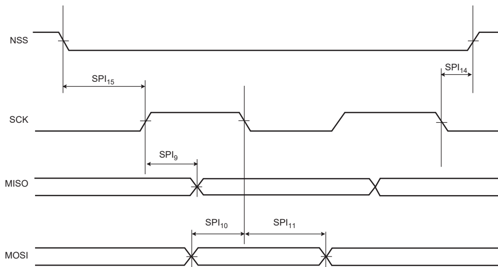
Figure 57-22. USART SPI Client Mode (Mode 0 or 3)
