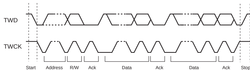
Figure 42-3. Transfer Format
