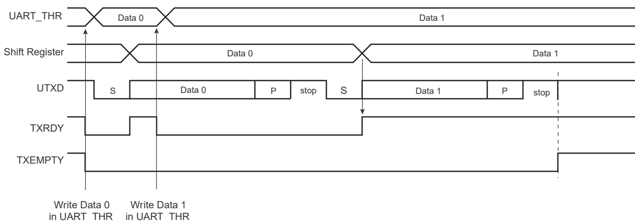
Figure 46-10. Transmitter Control
