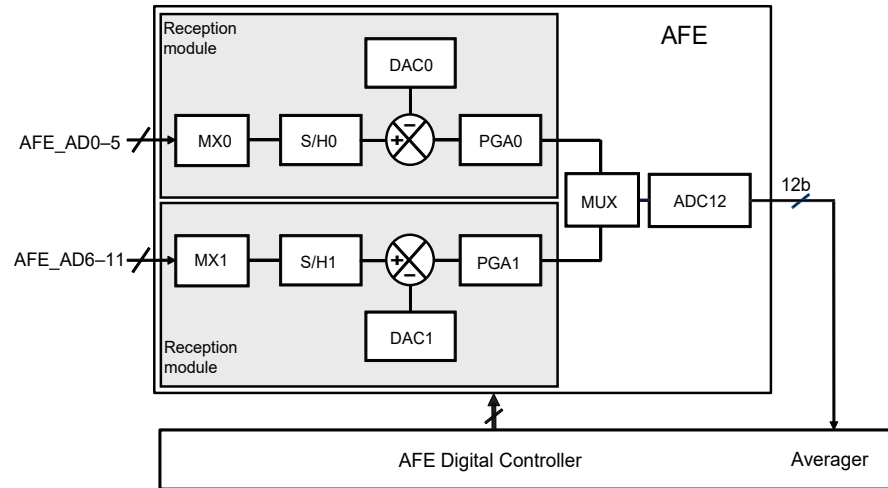
Figure 51-15. Single-ended Mode AFE
