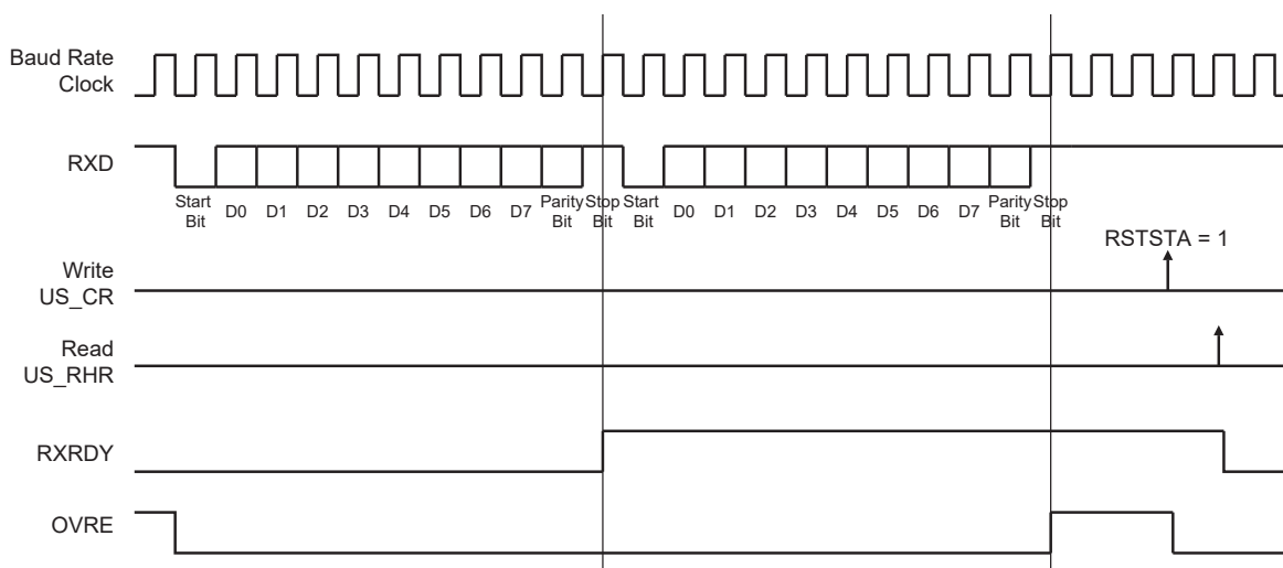
Figure 45-20. Receiver Status
