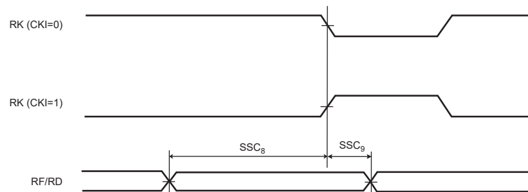
Figure 57-31. SSC Receiver RK and RF in Input
