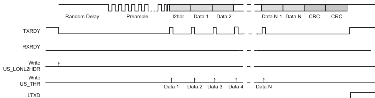
Figure 45-61. Tx Frame
