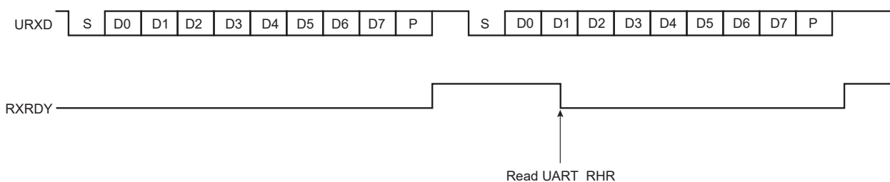
Figure 46-5. Receiver Ready
