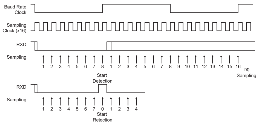
Figure 45-11. Asynchronous Start Detection
