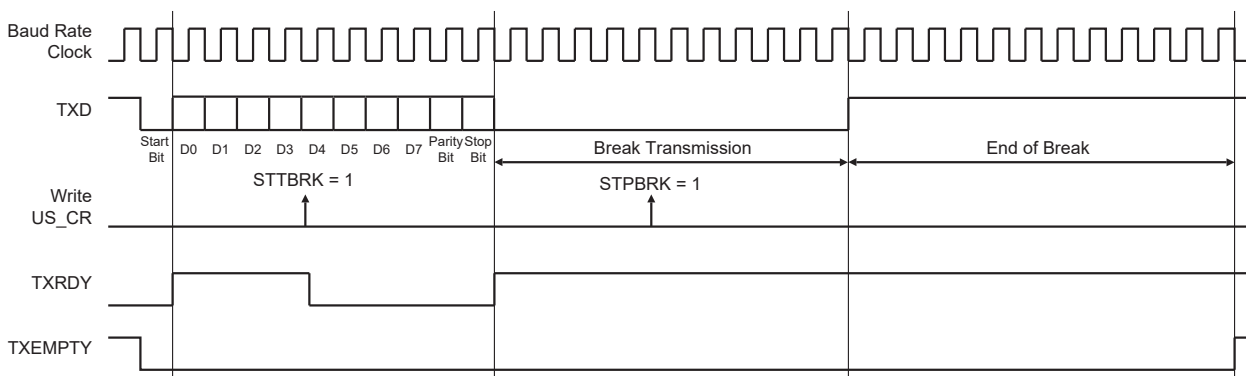
Figure 45-25. Break Transmission
