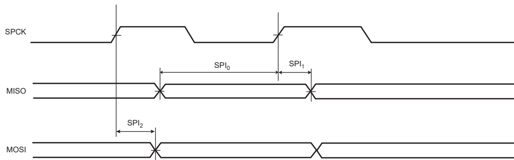
Figure 57-14. SPI Host Mode with (CPOL= NCPHA = 0) or (CPOL= NCPHA= 1)
