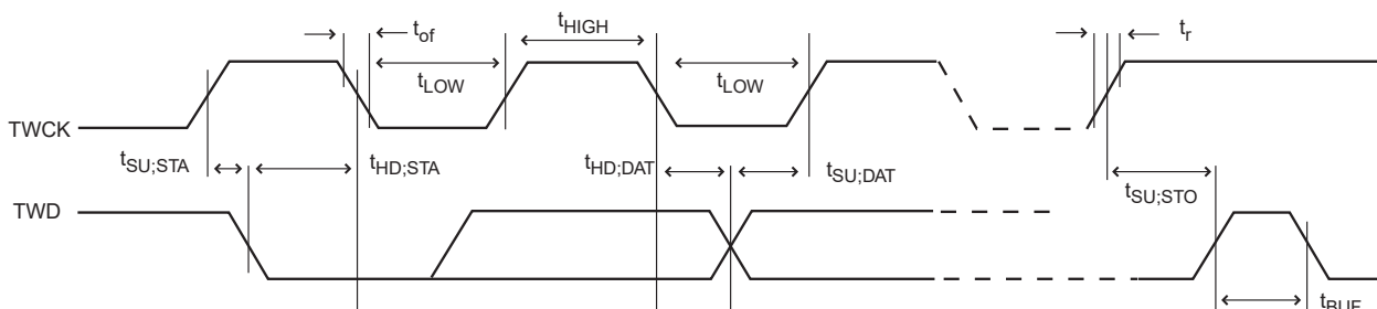
Figure 57-23. Two-wire Serial Bus Timing
