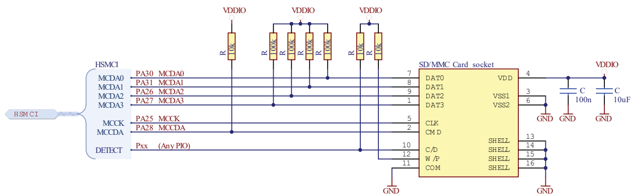
Figure 59-4. Schematic Example with SD/MMC Card Interface
