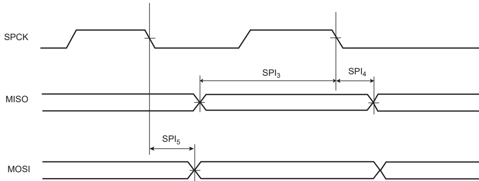
Figure 57-15. SPI Host Mode with (CPOL = 0 and NCPHA=1) or (CPOL=1 and NCPHA=0)
