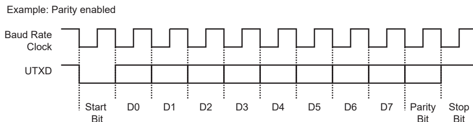
Figure 46-9. Character Transmission
