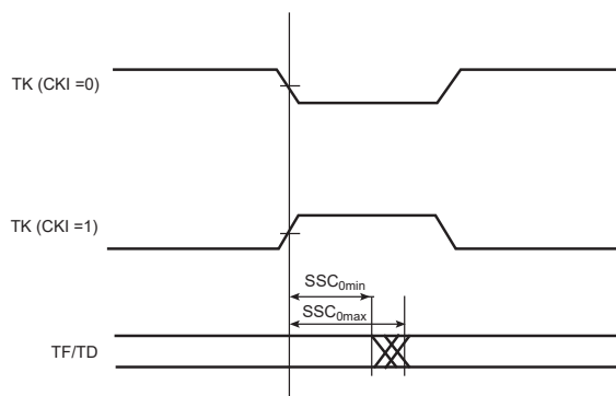
Figure 57-35. Min and Max Access Time of Output Signals
