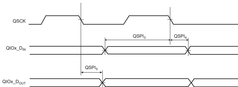
Figure 57-12. QSPI Host Mode with (CPOL = CPHA = 0) or (CPOL = CPHA = 1)
