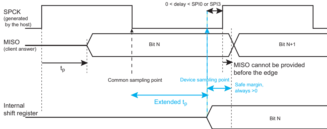
Figure 57-14. SPI Host Mode with (CPOL= NCPHA = 0) or (CPOL= NCPHA= 1)
