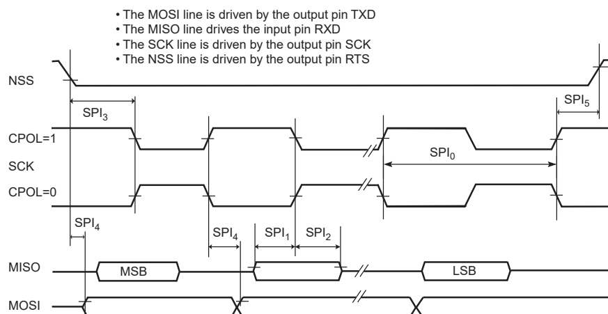
Figure 57-21. USART SPI Client Mode (Mode 1 or 2)
