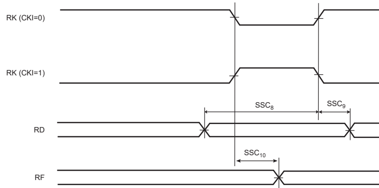
Figure 57-33. SSC Receiver, RK and RF in Output
