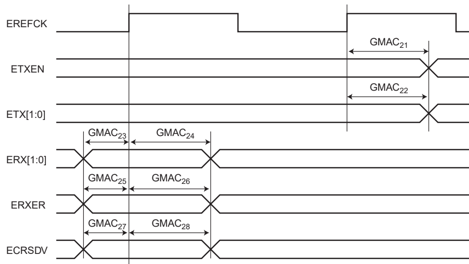
Figure 57-26. GMAC RMII Mode Signals
