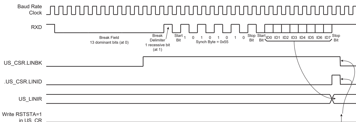
Figure 45-40. Header Reception
