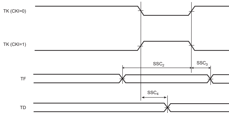
Figure 57-29. SSC Transmitter, TK in Output and TF in Input
