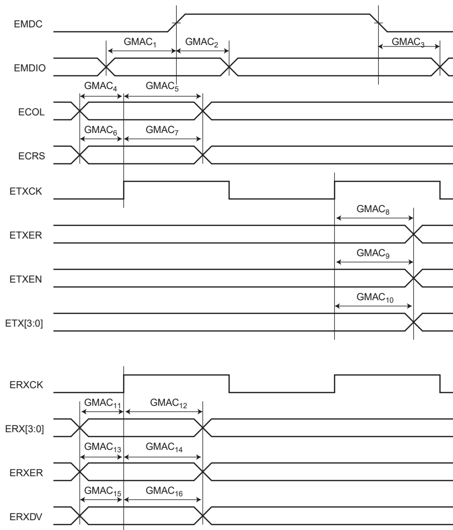
Figure 57-25. GMAC MII Mode Signals
