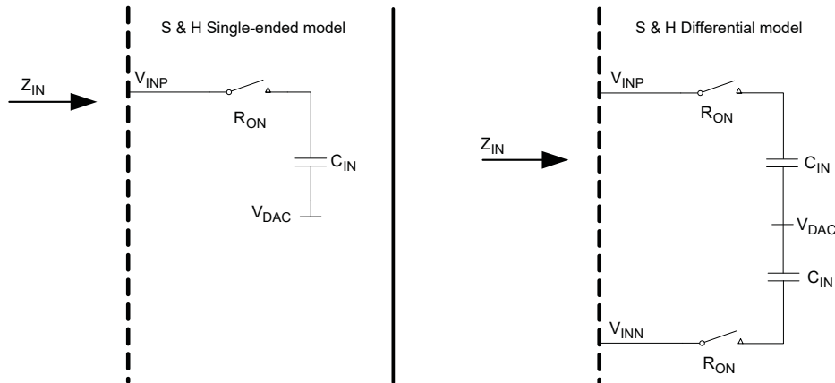
Figure 51-19. Input Channel Model
