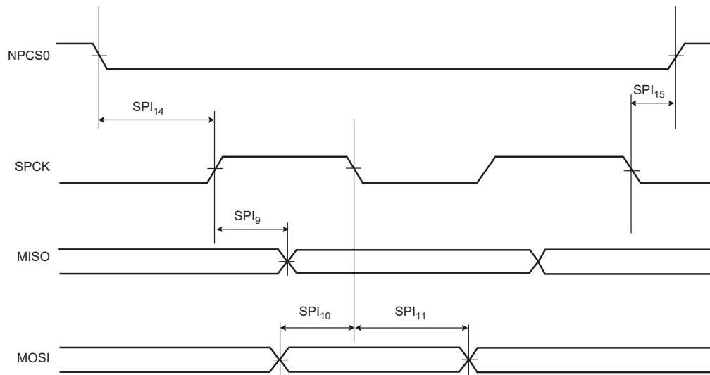
Figure 57-17. SPI Client Mode with (CPOL = NCPHA = 0) or (CPOL= NCPHA= 1)
