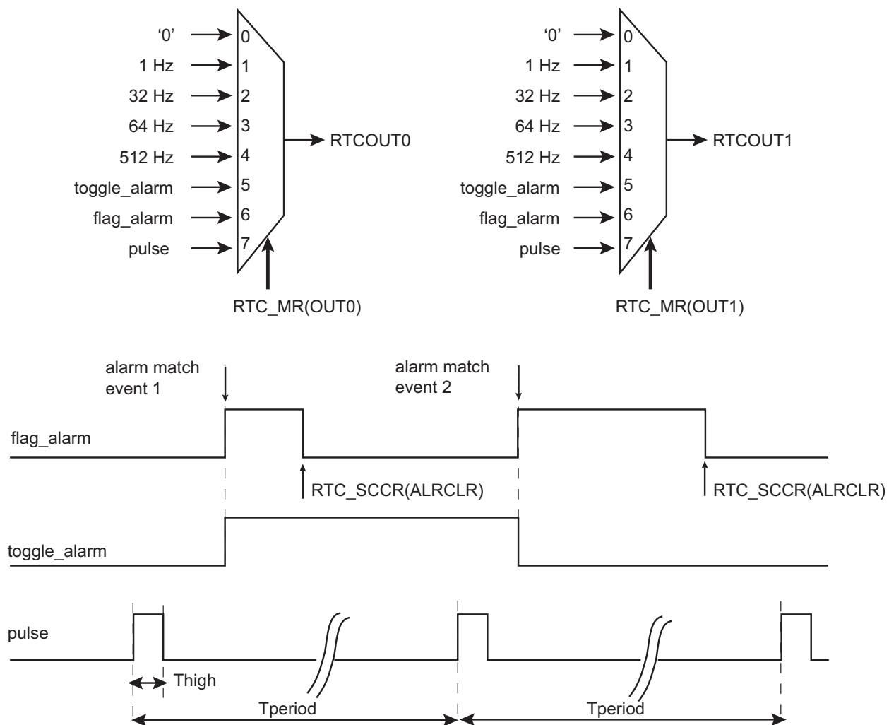
Figure 27-6. Waveform Generation
