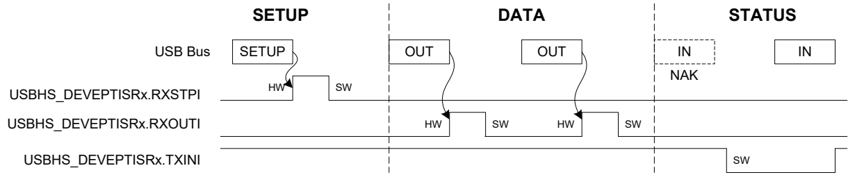
Figure 38-9. Control Write
