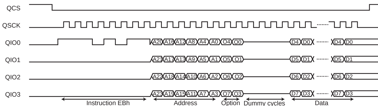
Figure 41-8. Instruction Frame
