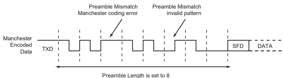
Figure 45-14. Preamble Pattern Mismatch
