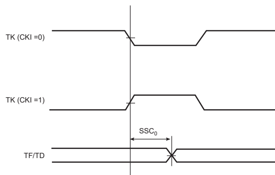
Figure 57-27. SSC Transmitter, TK and TF in Output
