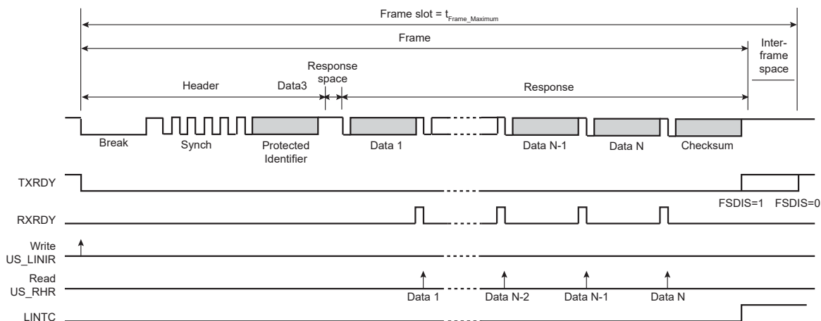
Figure 45-47. Host Node Configuration, NACT = IGNORE
