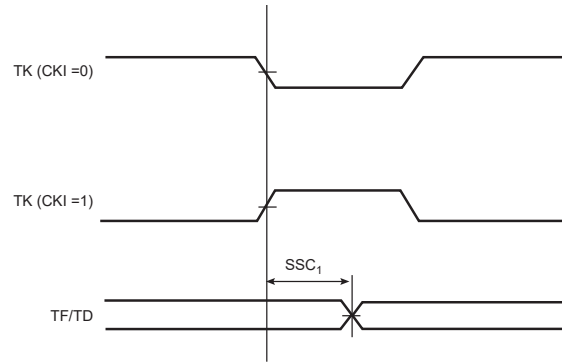
Figure 57-29. SSC Transmitter, TK in Output and TF in Input
