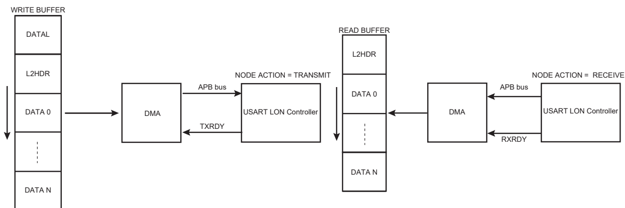
Figure 45-63. DMAM = 1
