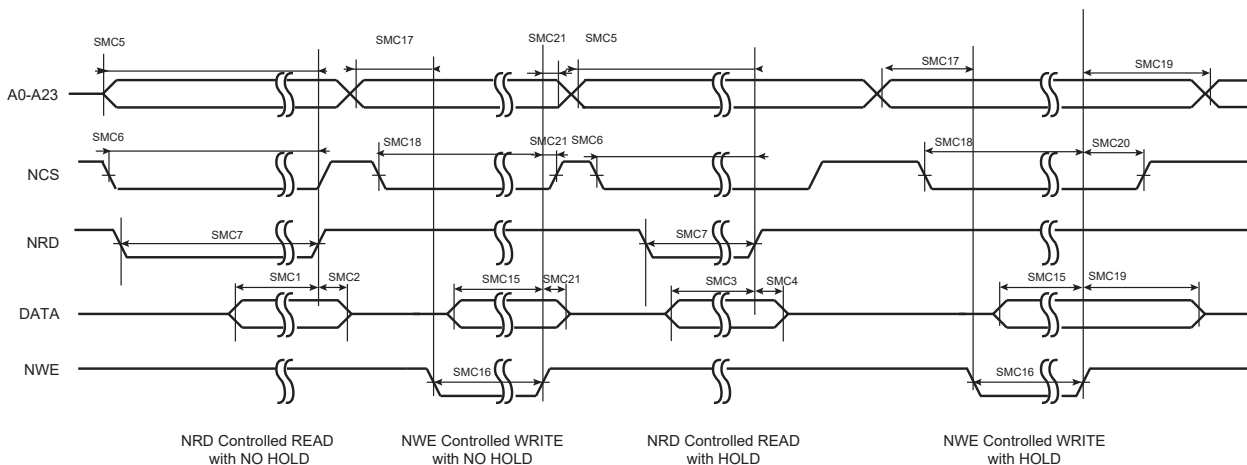
Figure 57-19. SMC Timings - NRD Controlled Read and NWE Controlled Write
