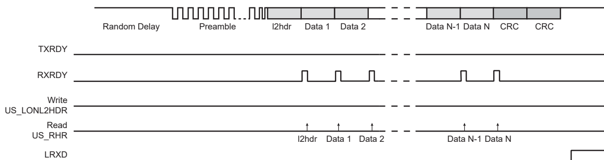
Figure 45-62. Rx Frame
