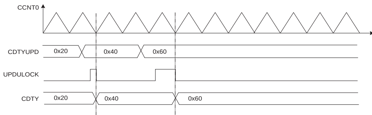
Figure 50-19. Method 1 (UPDM = 0)
