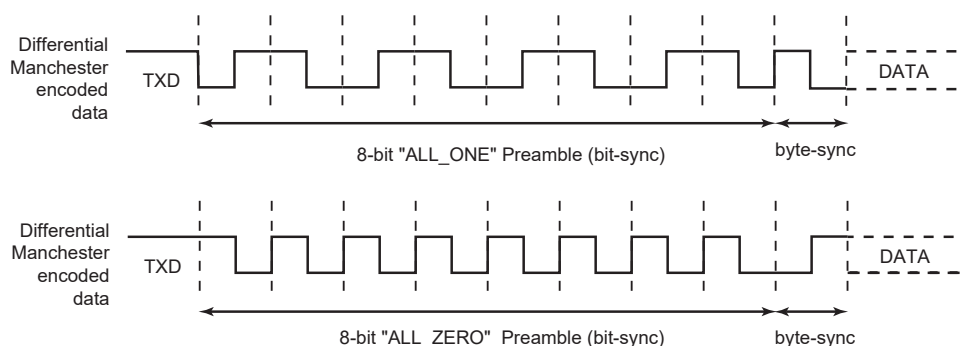
Figure 45-57. Preamble Patterns
