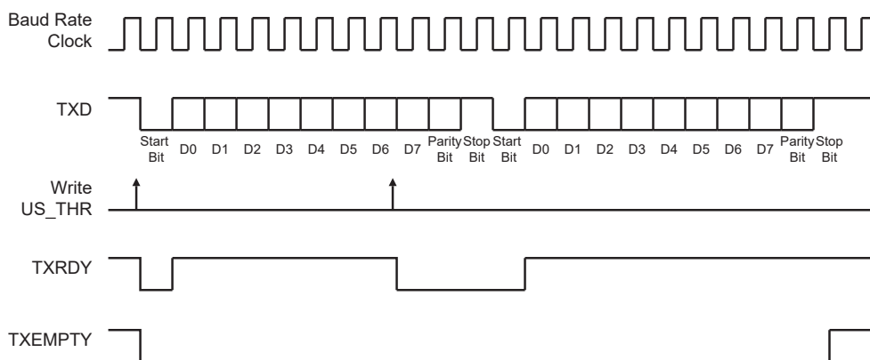
Figure 45-6. Transmitter Status
