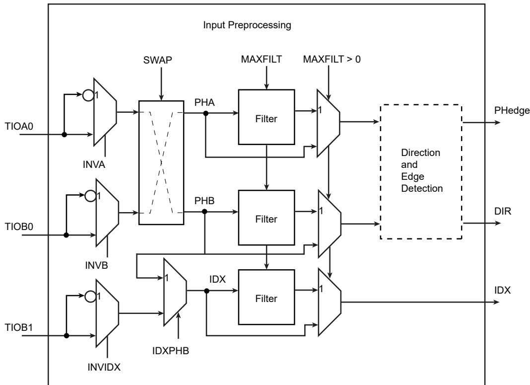
Figure 49-18. Input Stage
