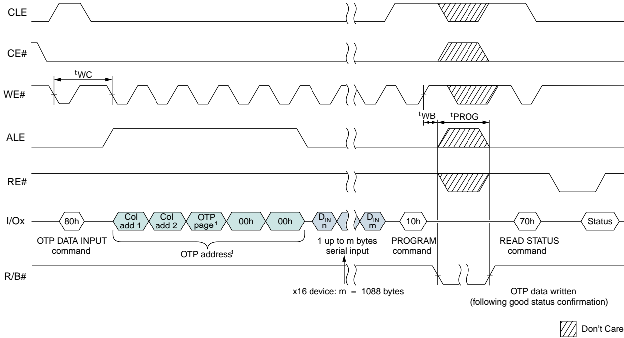
Figure 67: OTP DATA PROGRAM (After Entering OTP Operation Mode)
