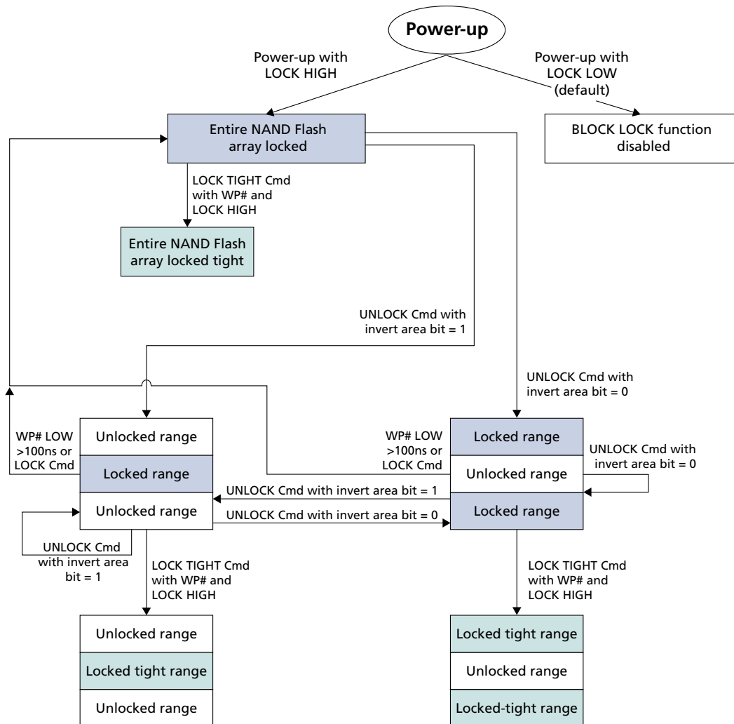
Figure 65: BLOCK LOCK Flowchart
