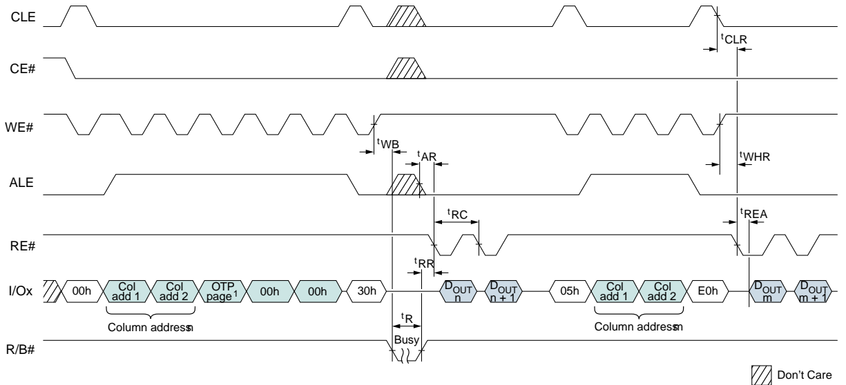
Figure 71: OTP DATA READ with RANDOM DATA READ Operation
