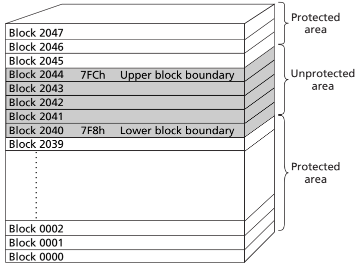
Figure 19: Flash Array Protected: Invert Area Bit = 1
