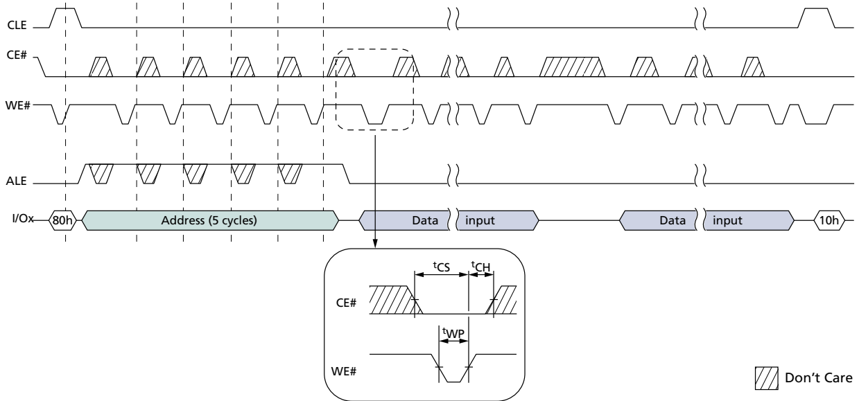
Figure 94: PROGRAM PAGE Operation with RANDOM DATA INPUT
