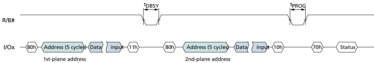
Figure 74: TWO-PLANE PROGRAM PAGE
