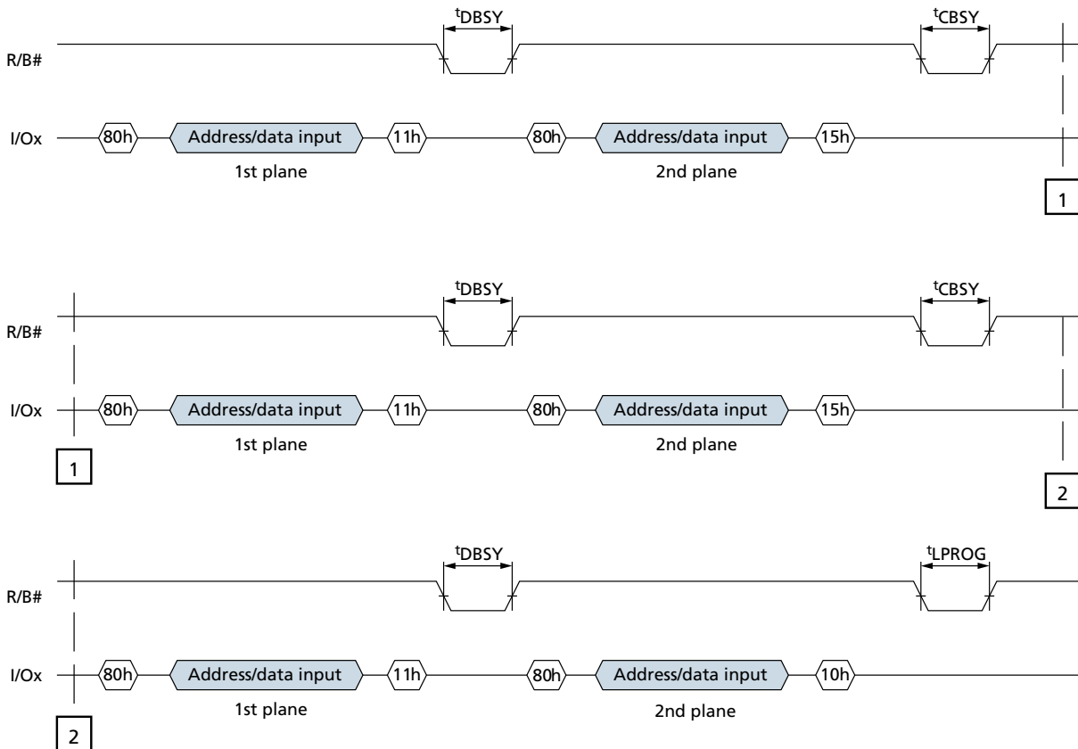
Figure 76: TWO-PLANE PROGRAM PAGE CACHE MODE
