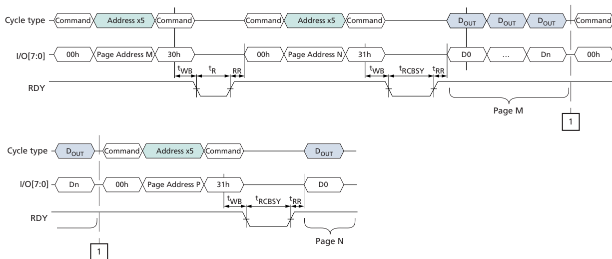
Figure 42: READ PAGE CACHE RANDOM (00h-31h) Operation
