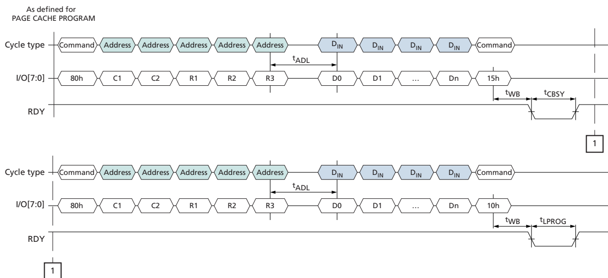
Figure 47: PROGRAM PAGE CACHE (80h–15h) Operation (End)
