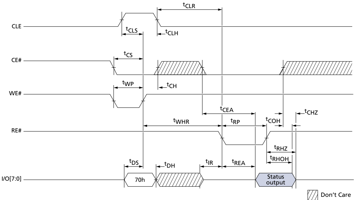
Figure 83: READ STATUS Cycle
