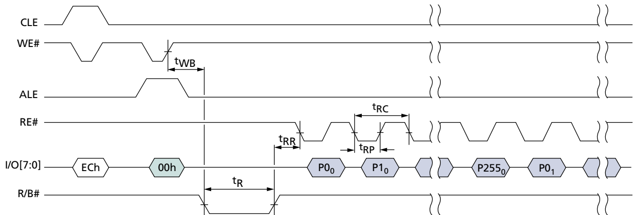
Figure 85: READ PARAMETER PAGE
