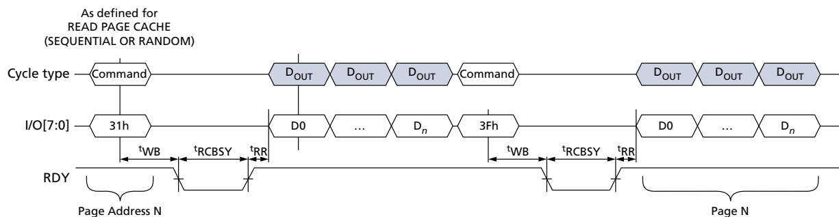
Figure 43: READ PAGE CACHE LAST (3Fh) Operation
