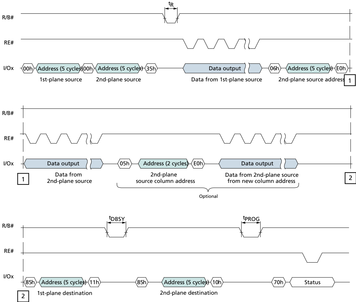
Figure 78: TWO-PLANE INTERNAL DATA MOVE with TWO-PLANE RANDOM DATA READ
