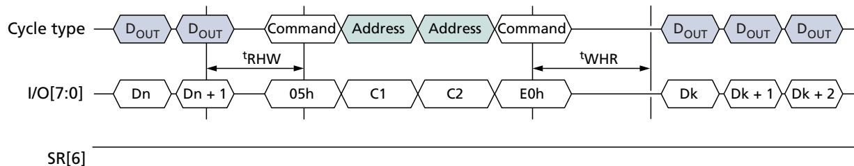
Figure 35: RANDOM DATA READ (05h-E0h) Operation
