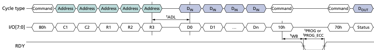
Figure 45: PROGRAM PAGE (80h-10h) Operation
