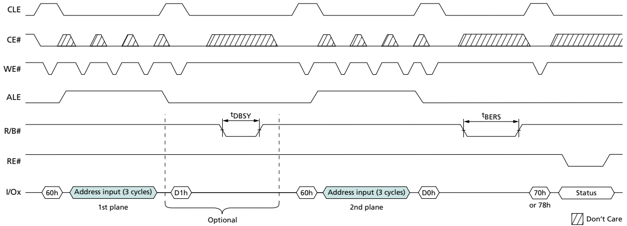
Figure 80: TWO-PLANE BLOCK ERASE
