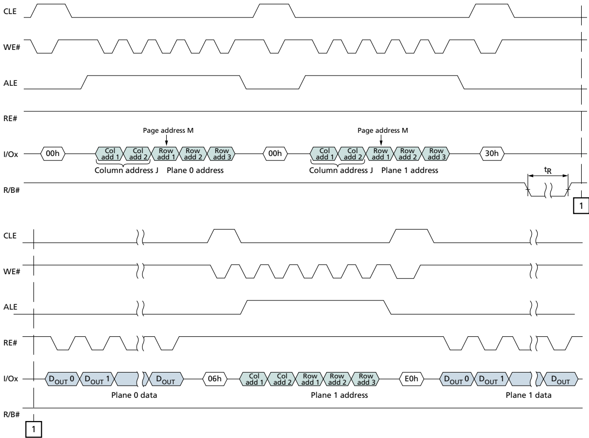
Figure 72: TWO-PLANE PAGE READ
