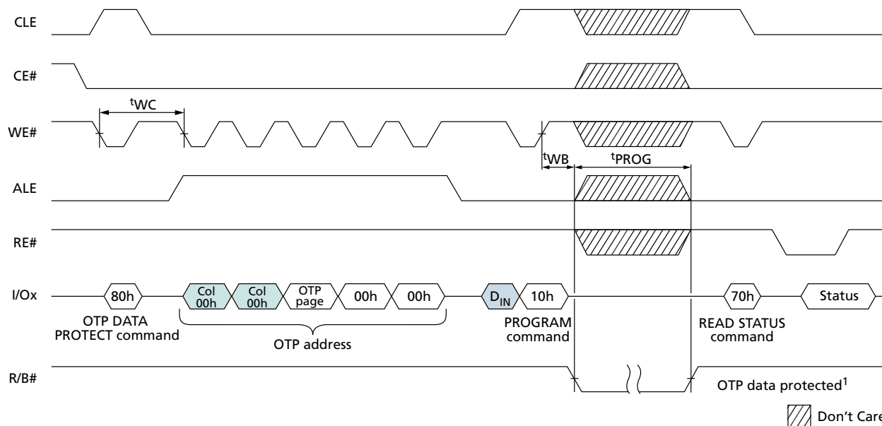
Figure 69: OTP DATA PROTECT Operation (After Entering OTP Protect Mode)
