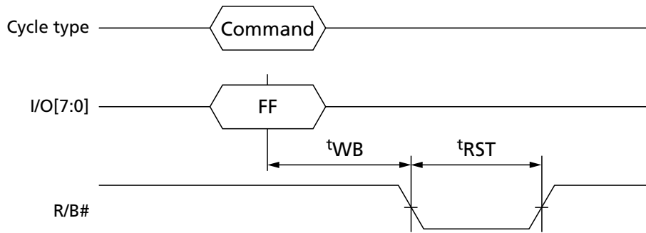
Figure 26: RESET (FFh) Operation
