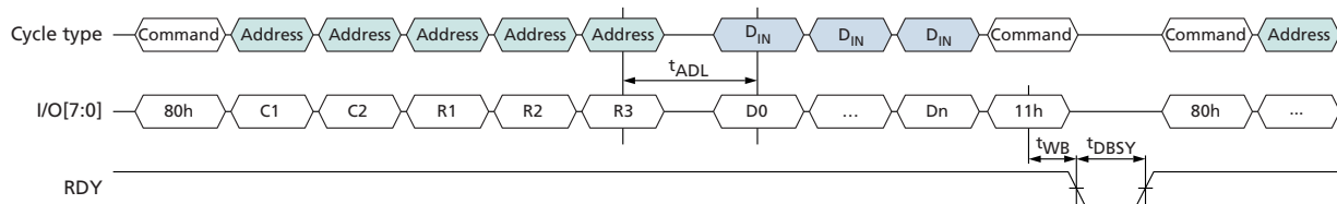
Figure 48: PROGRAM PAGE TWO-PLANE (80h–11h) Operation
