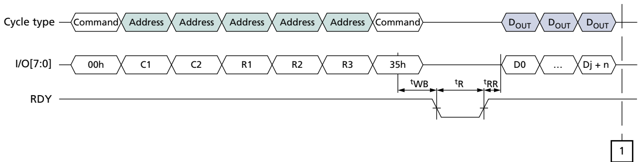
Figure 52: READ FOR INTERNAL DATA MOVE (00h-35h) with RANDOM DATA READ (05h-E0h)
