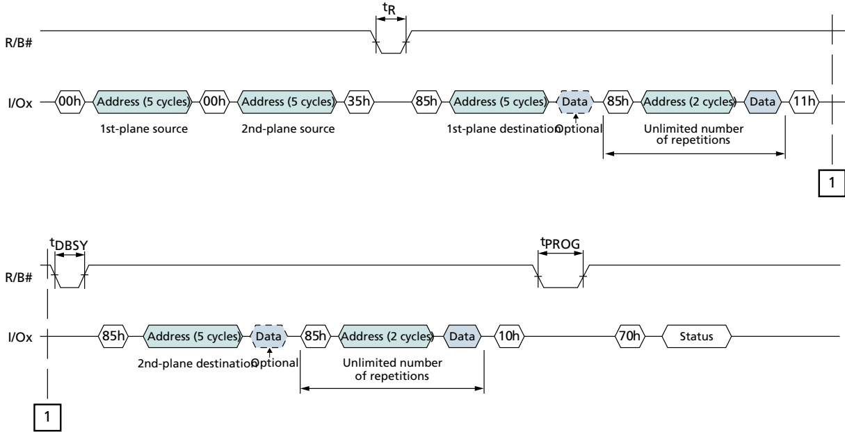
Figure 79: TWO-PLANE INTERNAL DATA MOVE with RANDOM DATA INPUT
