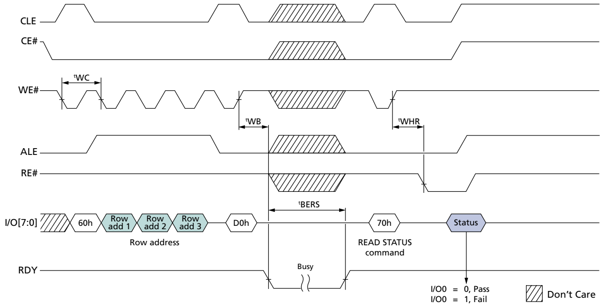
Figure 98: ERASE BLOCK Operation
