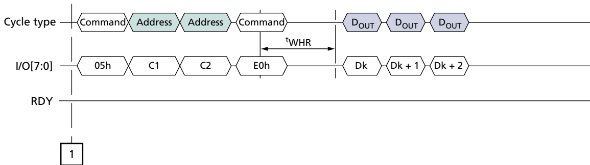
Figure 53: INTERNAL DATA MOVE (85h-10h) with Internal ECC Enabled
