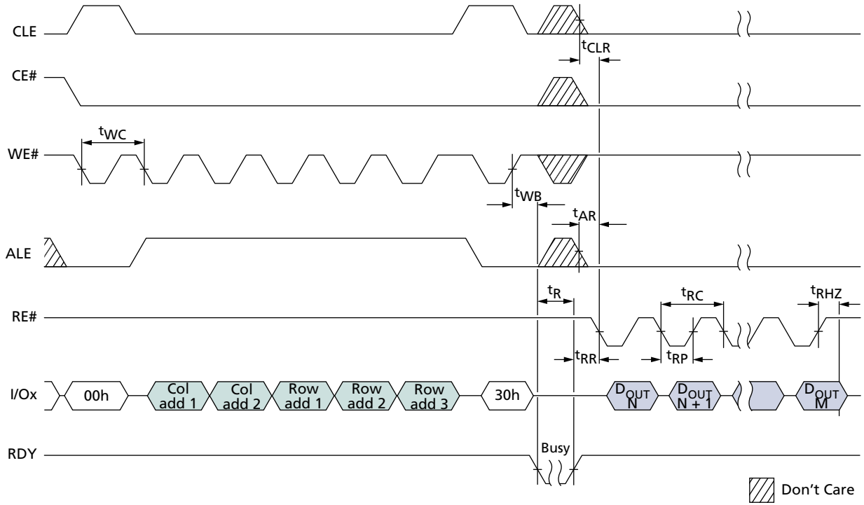
Figure 87: READ PAGE Operation with CE# "Don't Care"
