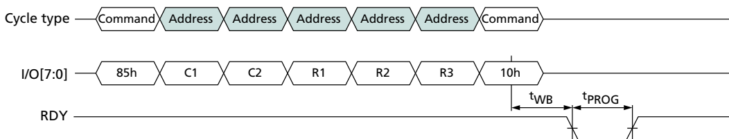
Figure 56: PROGRAM FOR INTERNAL DATA MOVE (85h-10h) with RANDOM DATA INPUT (85h)
