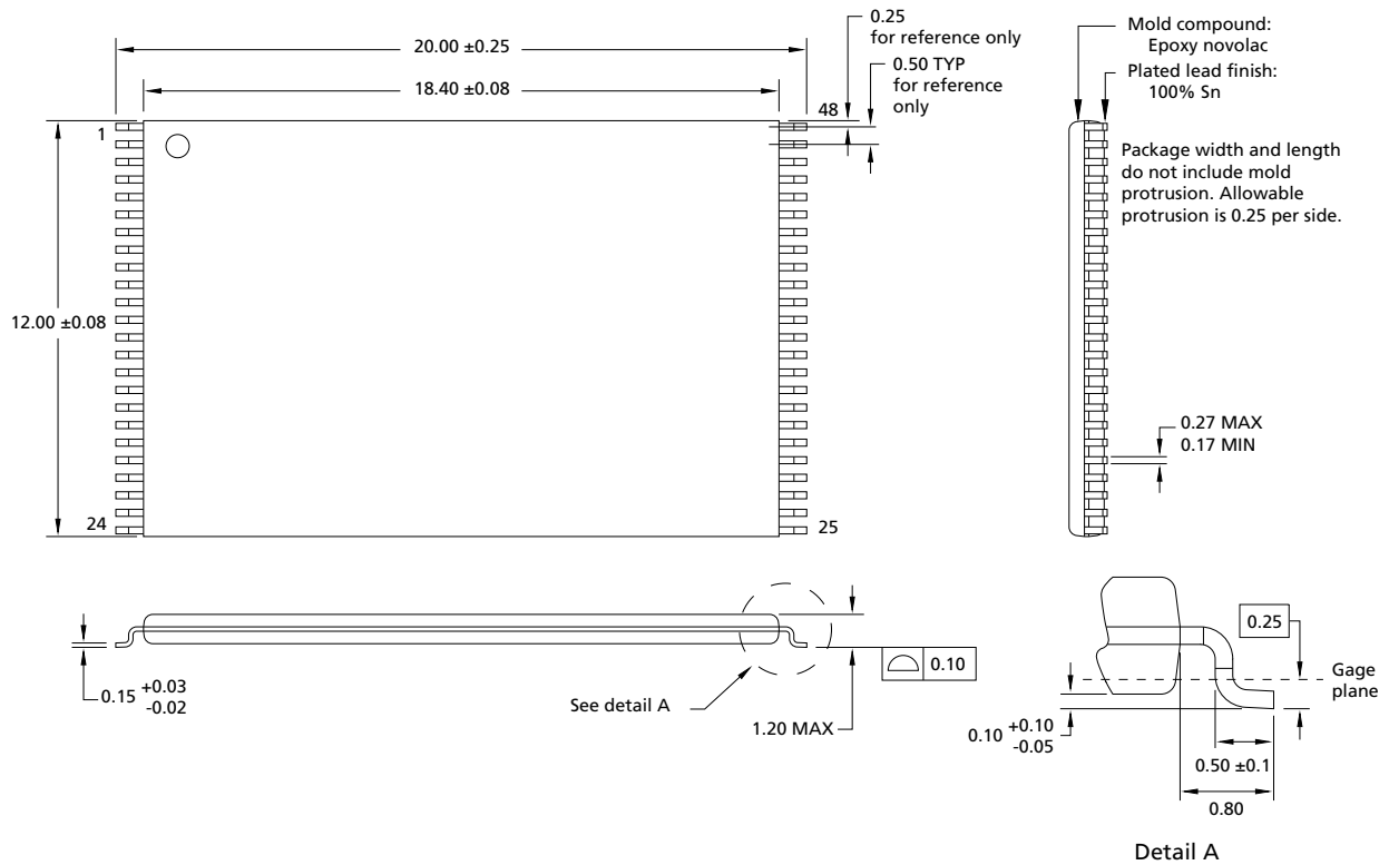
Figure 4: 48-Pin TSOP – Type 1, CPL (WP)
