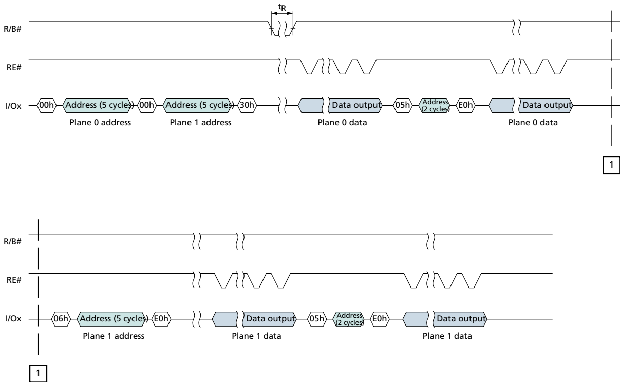
Figure 73: TWO-PLANE PAGE READ with RANDOM DATA READ
