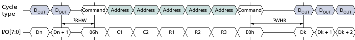
Figure 36: RANDOM DATA READ TWO-PLANE (06h-E0h) Operation
