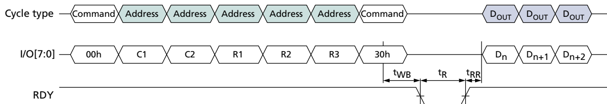
Figure 39: READ PAGE (00h-30h) Operation
