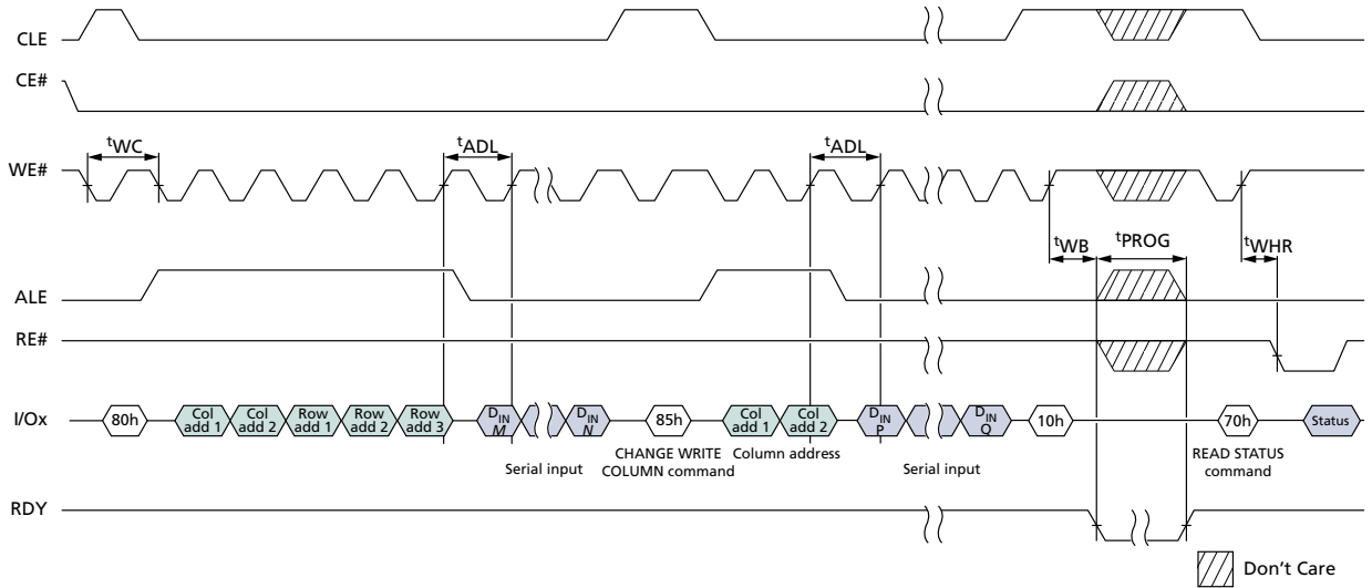
Figure 94: PROGRAM PAGE Operation with RANDOM DATA INPUT
