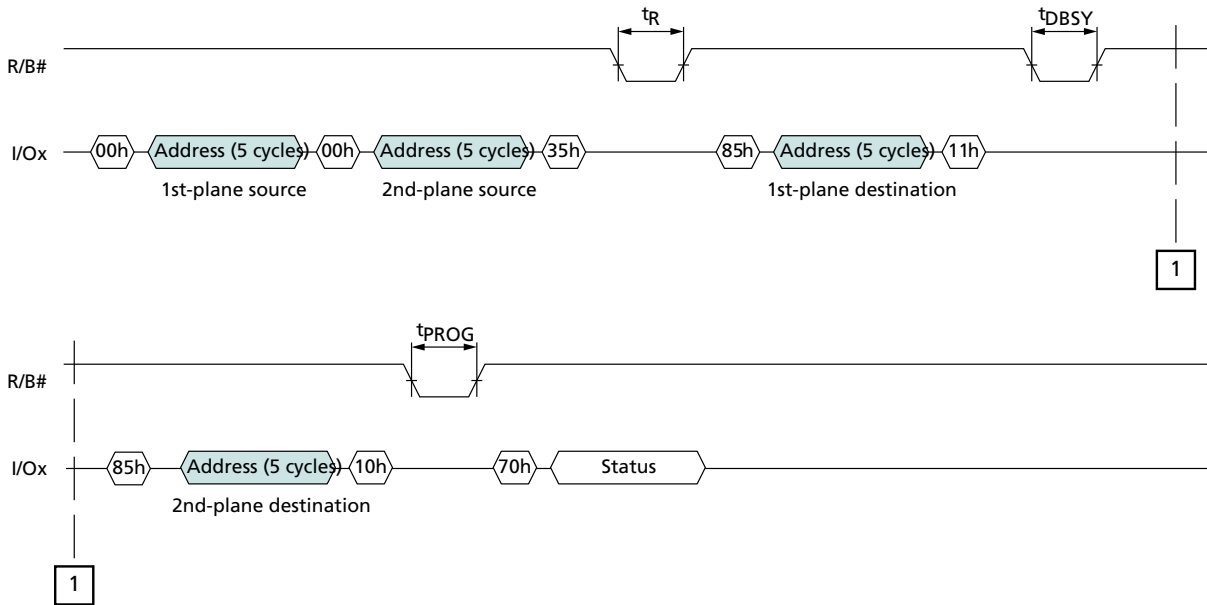
Figure 77: TWO-PLANE INTERNAL DATA MOVE
