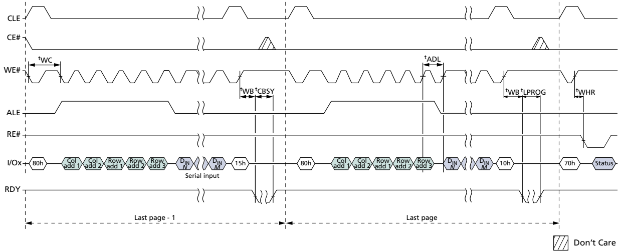
Figure 96: PROGRAM PAGE CACHE Ending on 15h
