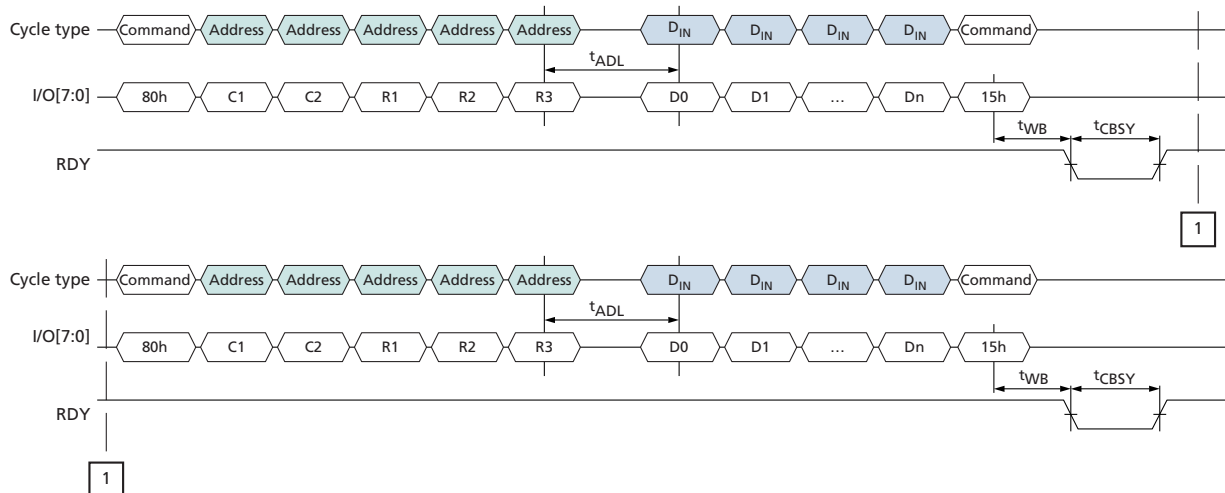
Figure 47: PROGRAM PAGE CACHE (80h–15h) Operation (End)
