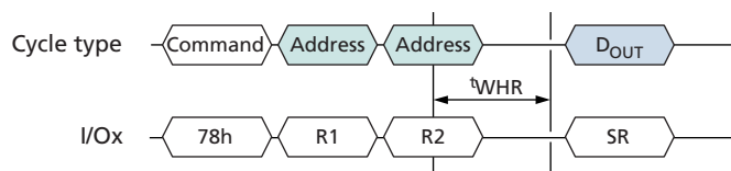
Figure 34: READ STATUS ENHANCED (78h) Operation
