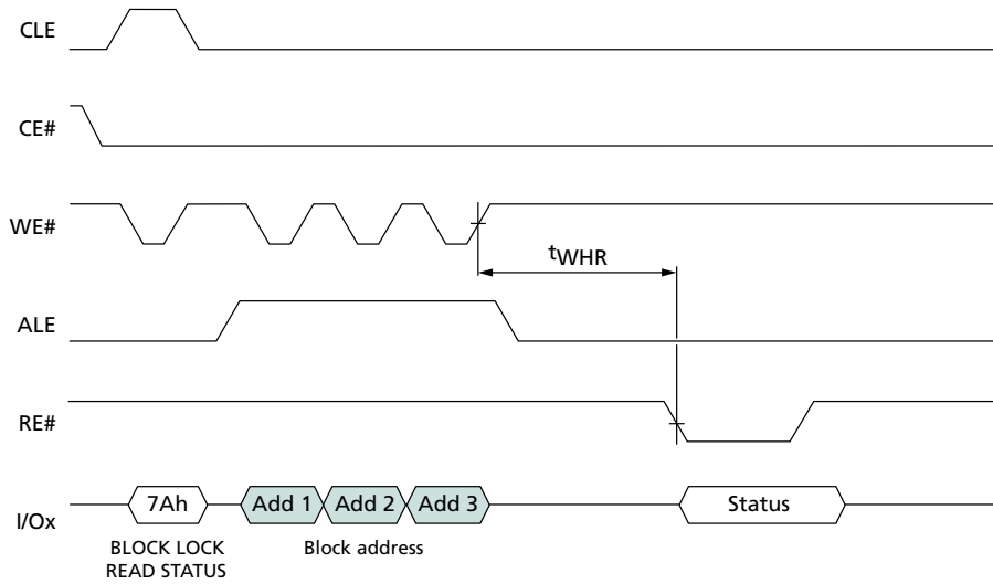
Figure 24: BLOCK LOCK READ STATUS
