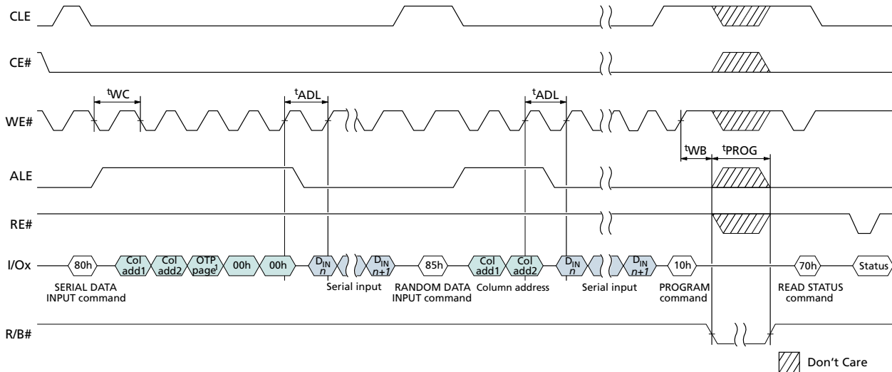
Figure 68: OTP DATA PROGRAM Operation with RANDOM DATA INPUT (After Entering OTP Operation Mode)
