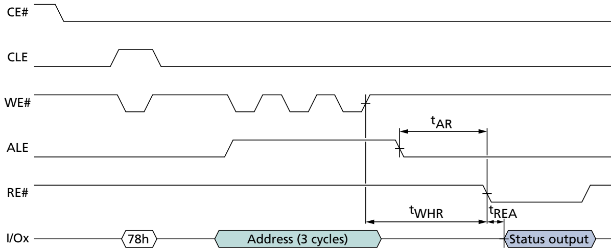
Figure 81: TWO-PLANE/MULTIPLE-DIE READ STATUS Cycle
