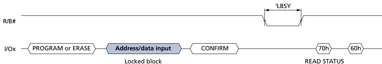
Figure 23: PROGRAM/ERASE Issued to Locked Block
