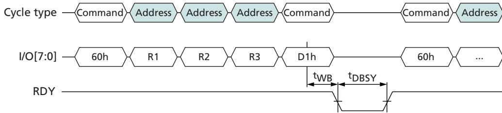
Figure 50: ERASE BLOCK TWO-PLANE (60h-D1h) Operation
