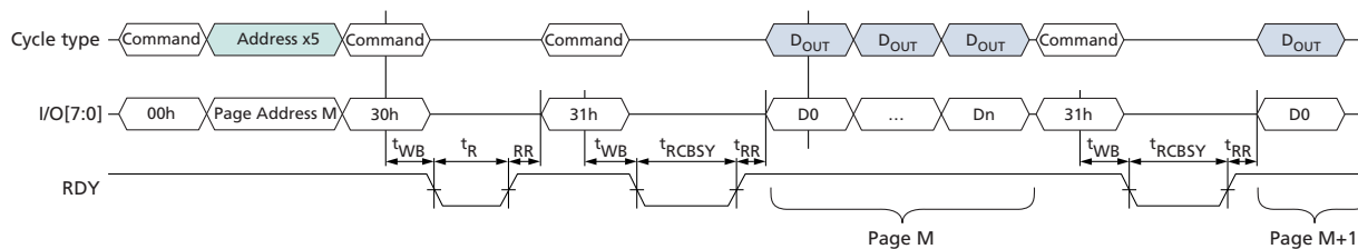
Figure 41: READ PAGE CACHE SEQUENTIAL (31h) Operation
