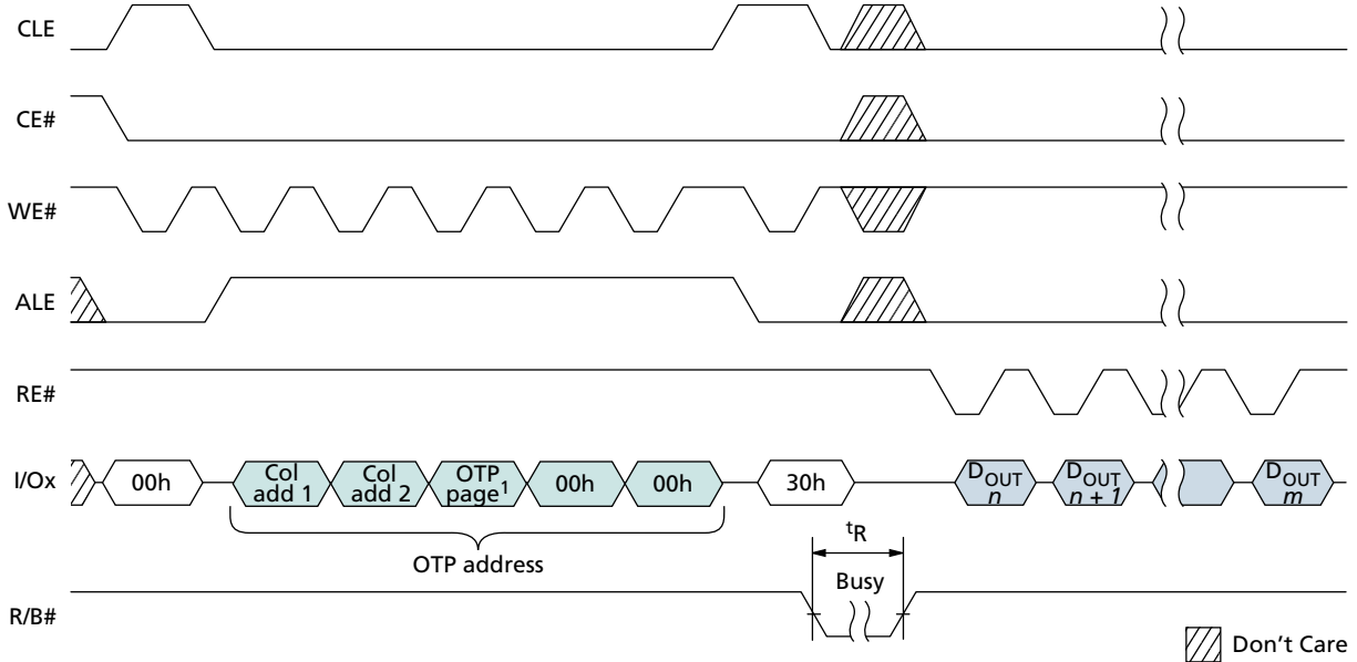
Figure 70: OTP DATA READ
