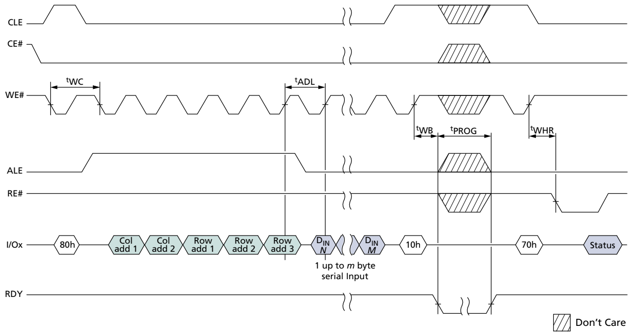
Figure 92: PROGRAM PAGE Operation
