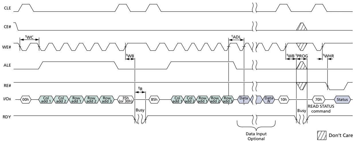
Figure 97: INTERNAL DATA MOVE
