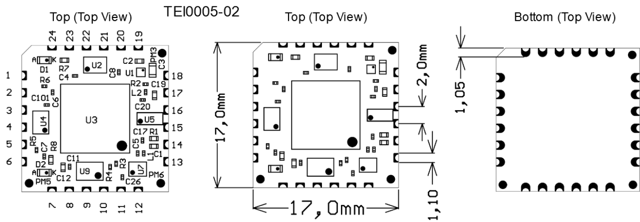
Figure 3: Physical Dimension
