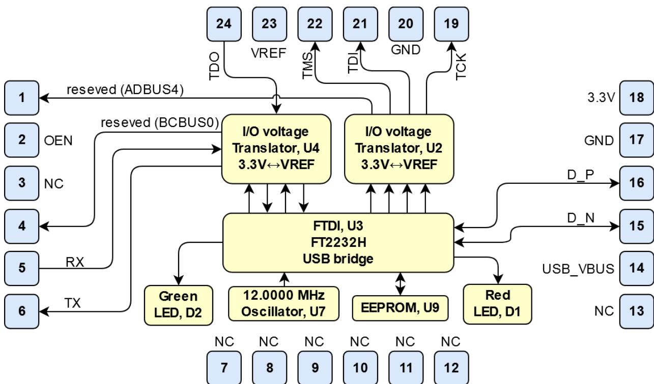
Figure 1: TEI0005 block diagram
