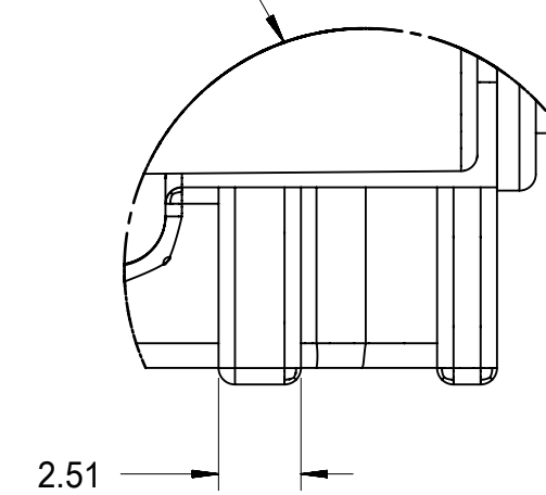
Partial1 SCALE 4:1
